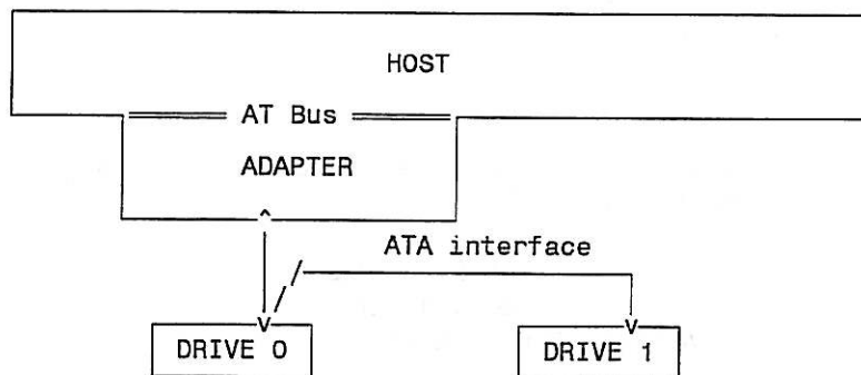
Figure 2 - Host bus adapter and peripheral devices
