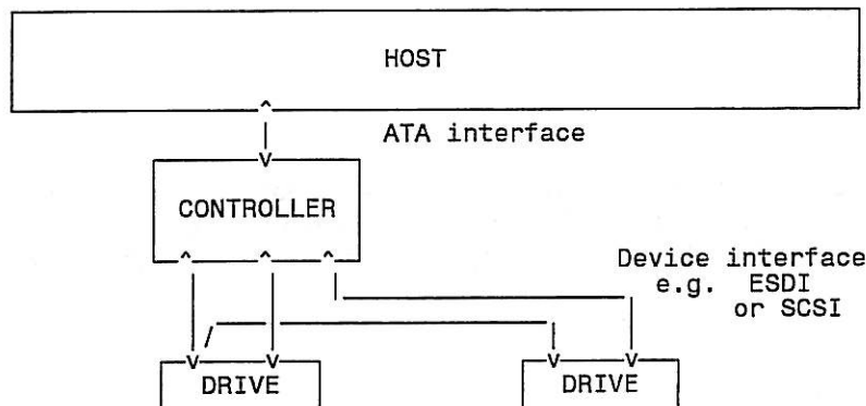
Figure 3 - ATA interface to controller and peripheral devices
