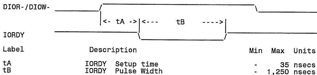
Figure 6 - PIO data transfer to/from drive
