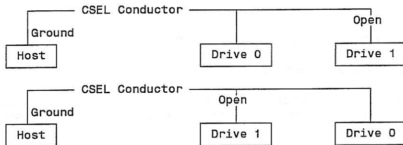
Figure 5 - Cable select
