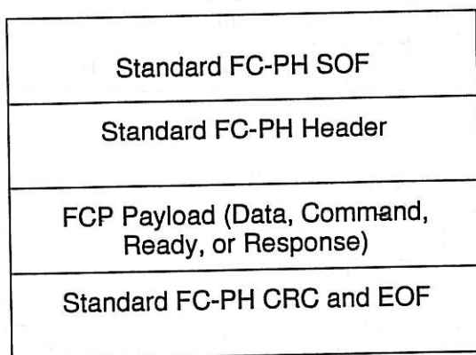
Figure 1 FCP Frame Format
