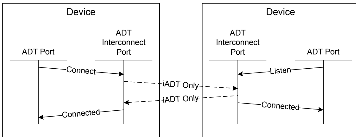
Figure 18 – Protocol services for establishing a connection
