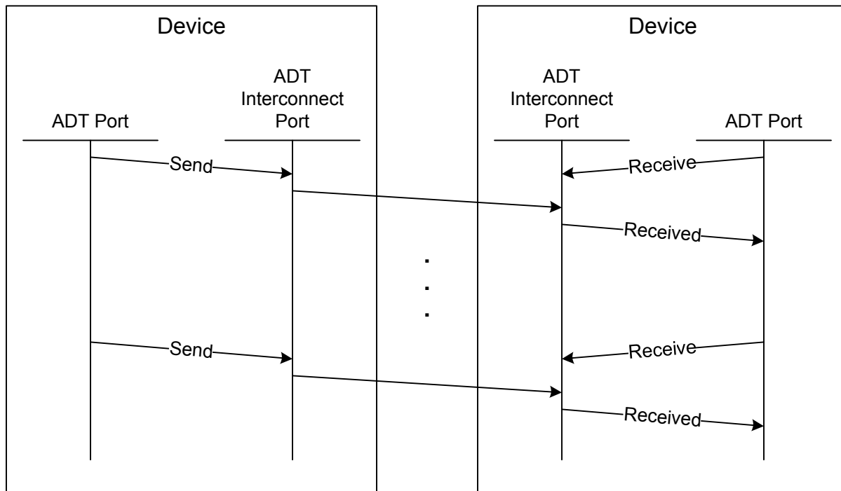
Figure 19 – Protocol services for transferring data
