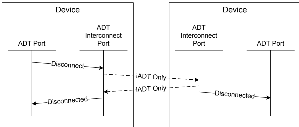
Figure 20 – Protocol services for closing a connection
