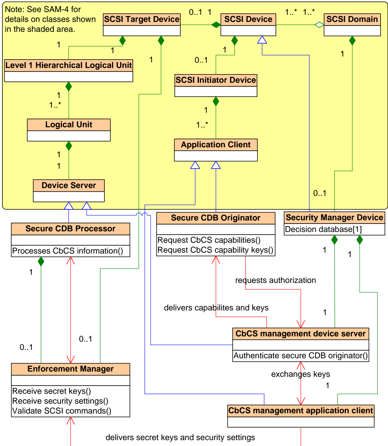
Figure 1 — CbCS class diagram
