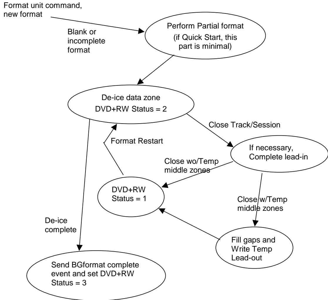
Figure 11 – Background Process Flow
