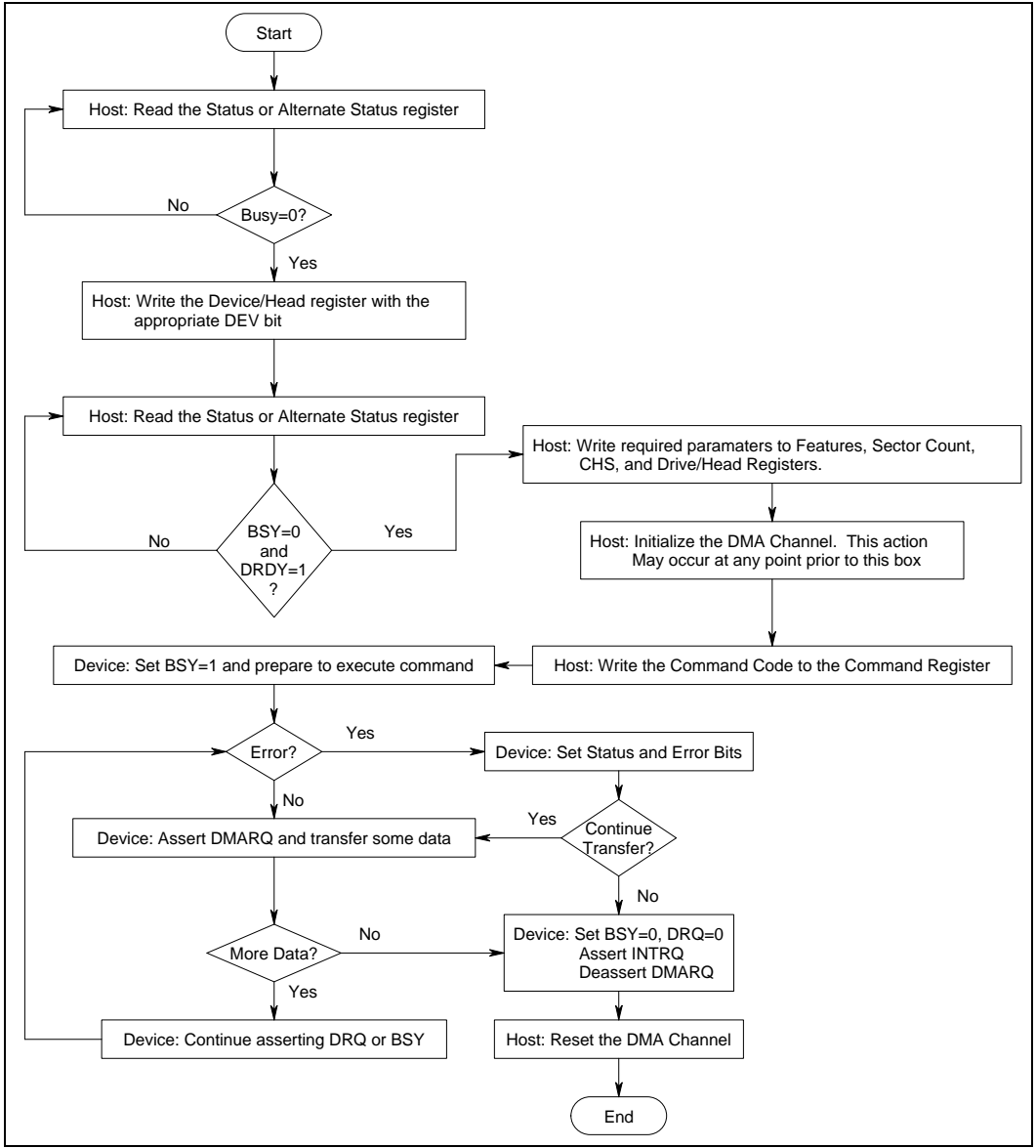
DMA Data Transfer Diagram
