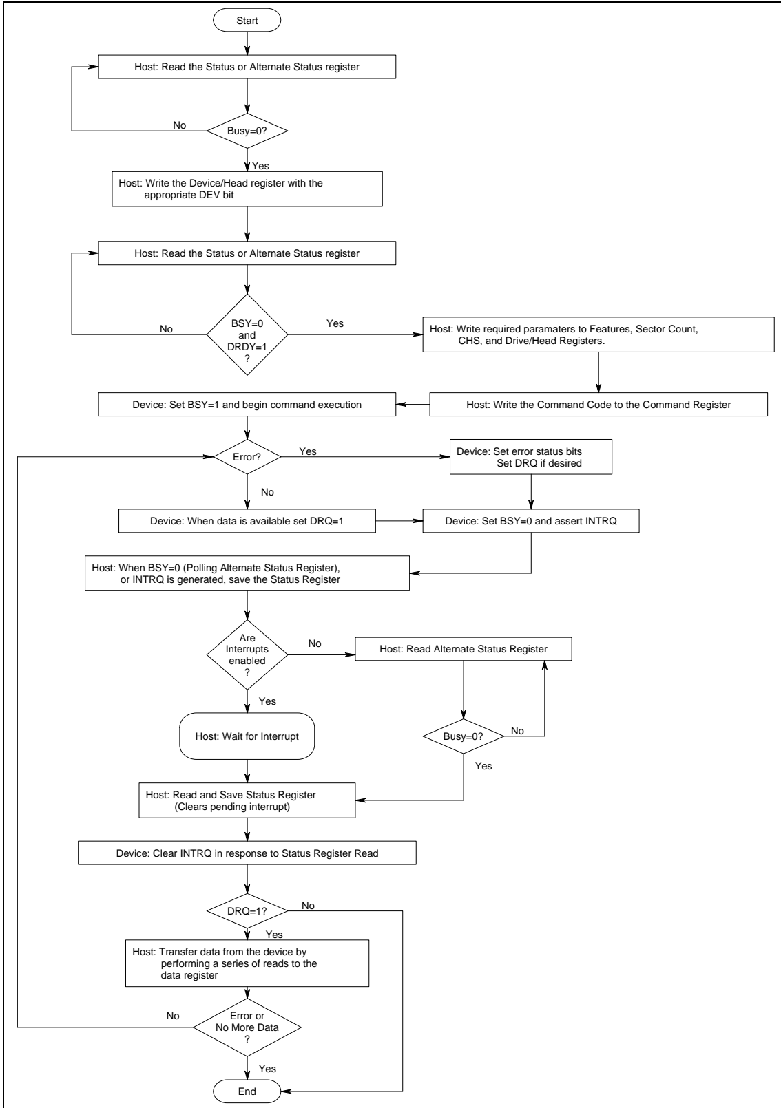
PIO Data Transfer IN Flowchart
