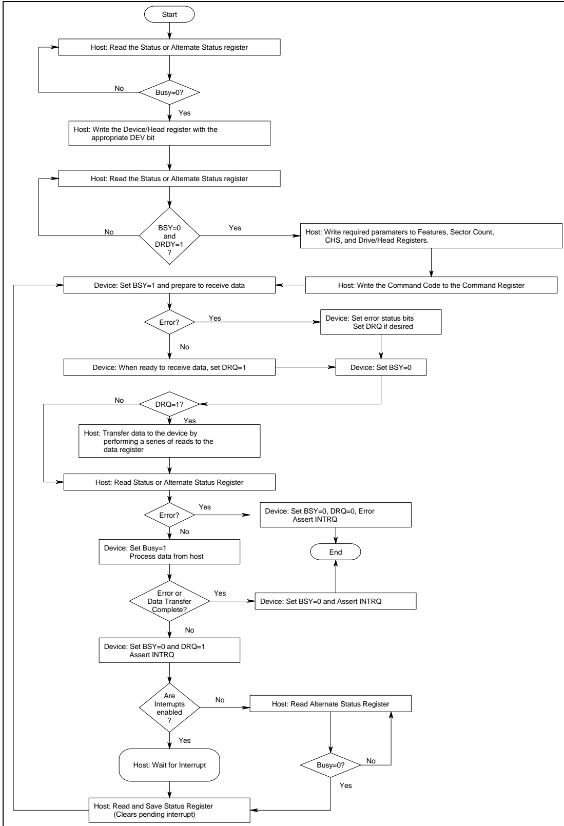
PIO Data Transfer Out Flowchart
