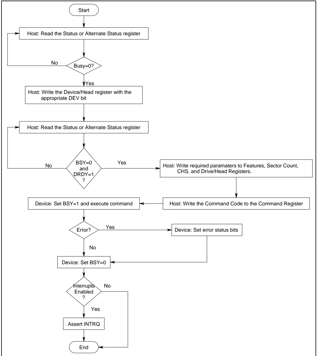
Non-data transfer Diagram
