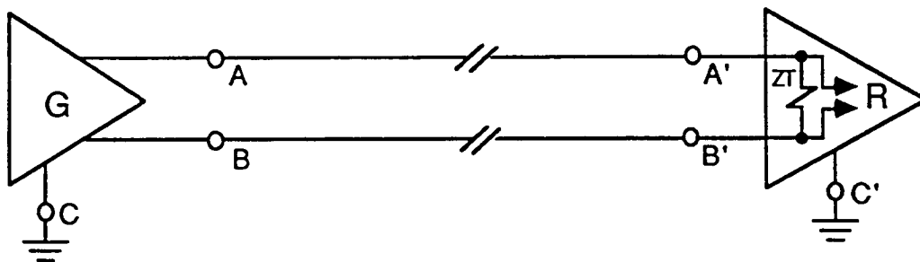
Figure 15 - Point-to-point application with internal termination
