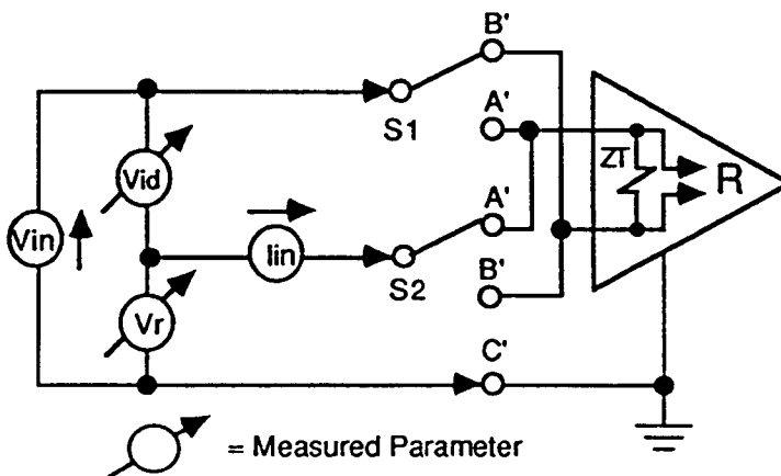
Figure 10 - Terminating receiver input current - voltage measurements
