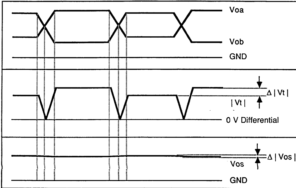
Figure B.1 - Generator output levels
