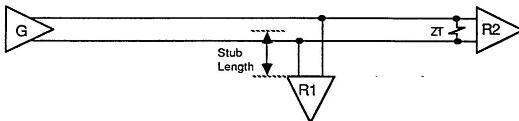
Figure 16 - Multiple receiver operation - multidrop application
