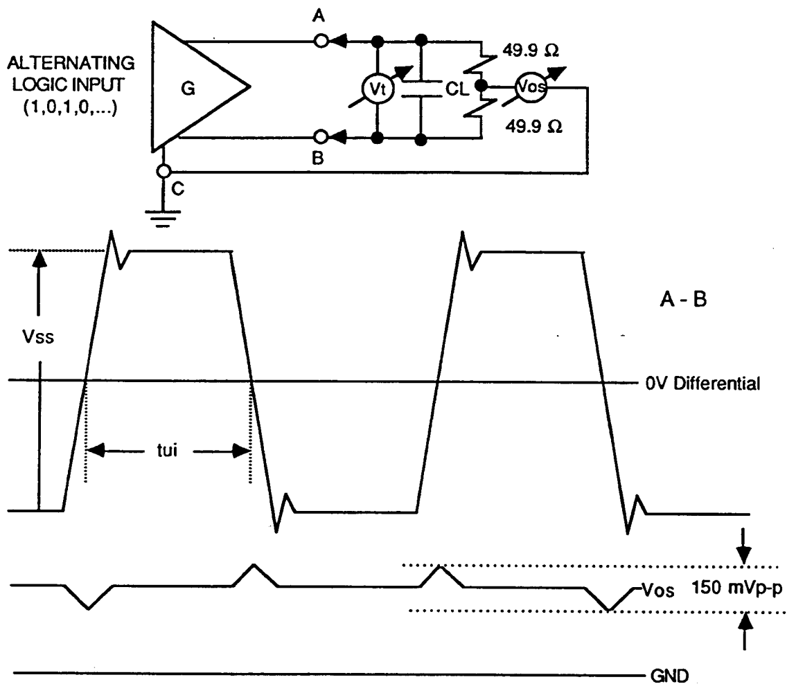
Figure 8 - Dynamic output signal balance waveform
