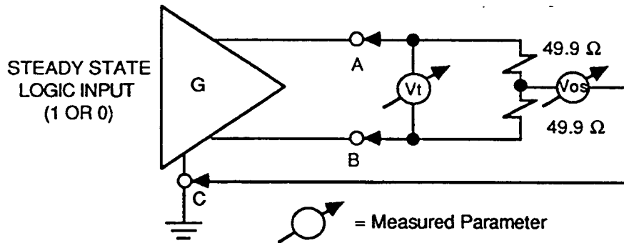
Figure 4 - Test termination measurements
