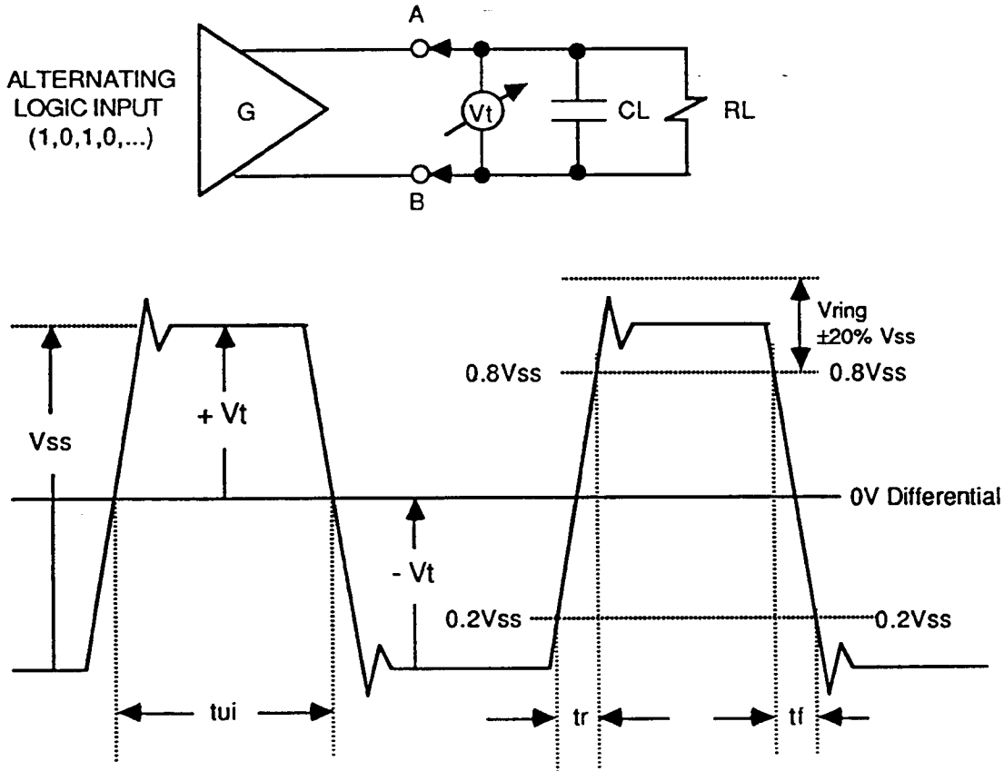
Figure 7 - Output signal waveform
