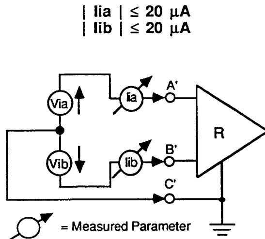
Figure 9 - Receiver input current - voltage measurements
