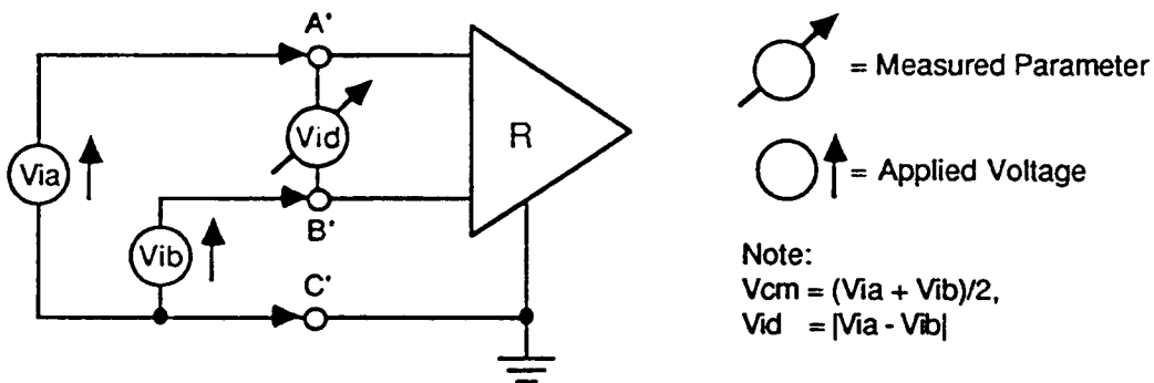
Figure 13 - Receiver input sensitivity test circuit
