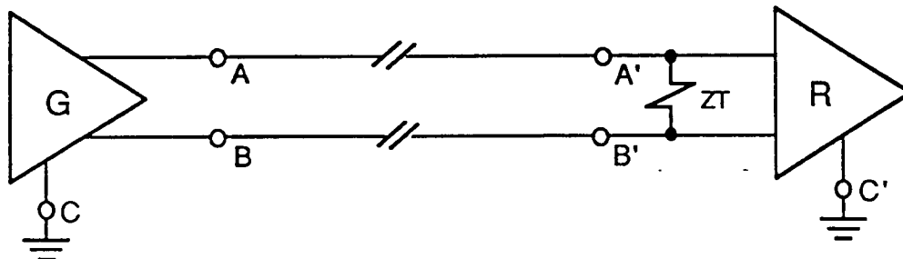
Figure 14 - Point-to-point application with external termination
