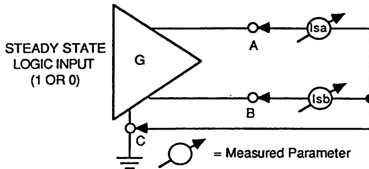
Figure 5 - Short-circuit measurements to circuit common
