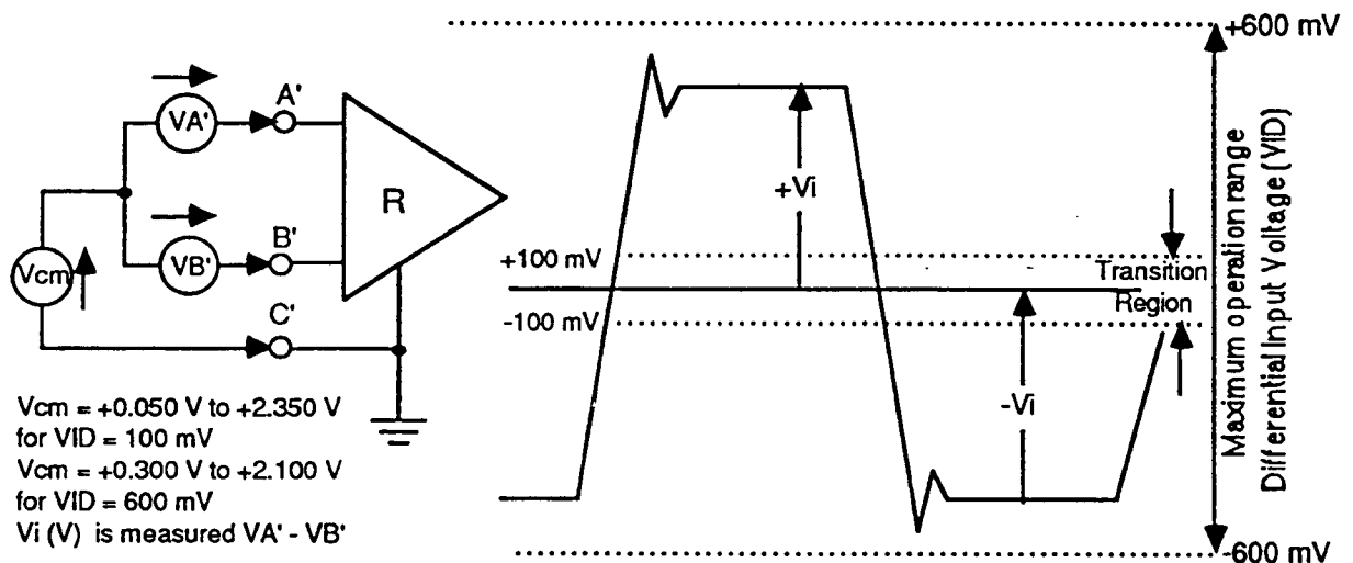
Figure 12 - Receiver input sensitivity measurements
