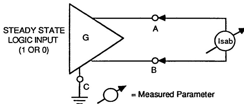
Figure 6 - Short-circuit measurements
