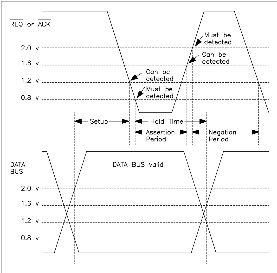
Figure B2 - Fast-20 timing measurements
