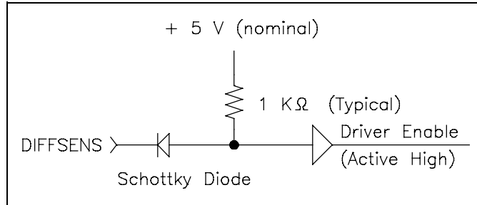
Figure 4 - Differential driver protection circuit
