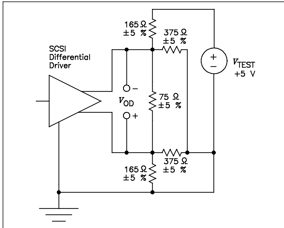
Figure 3 - Differential test circuit
