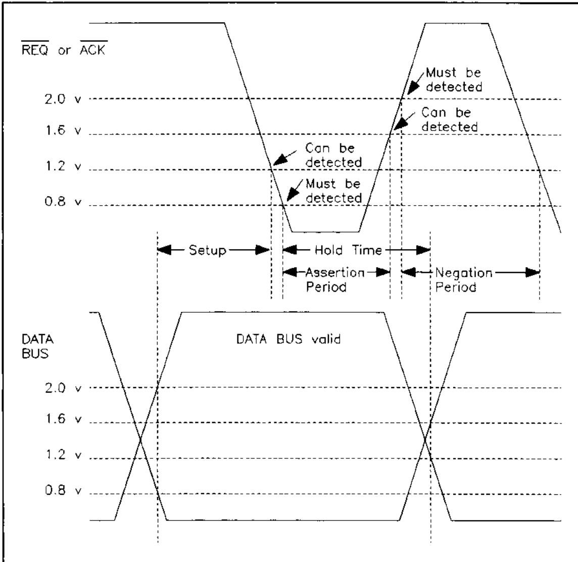
Figure B2 - Ultra Setup and hold timing for single-ended
