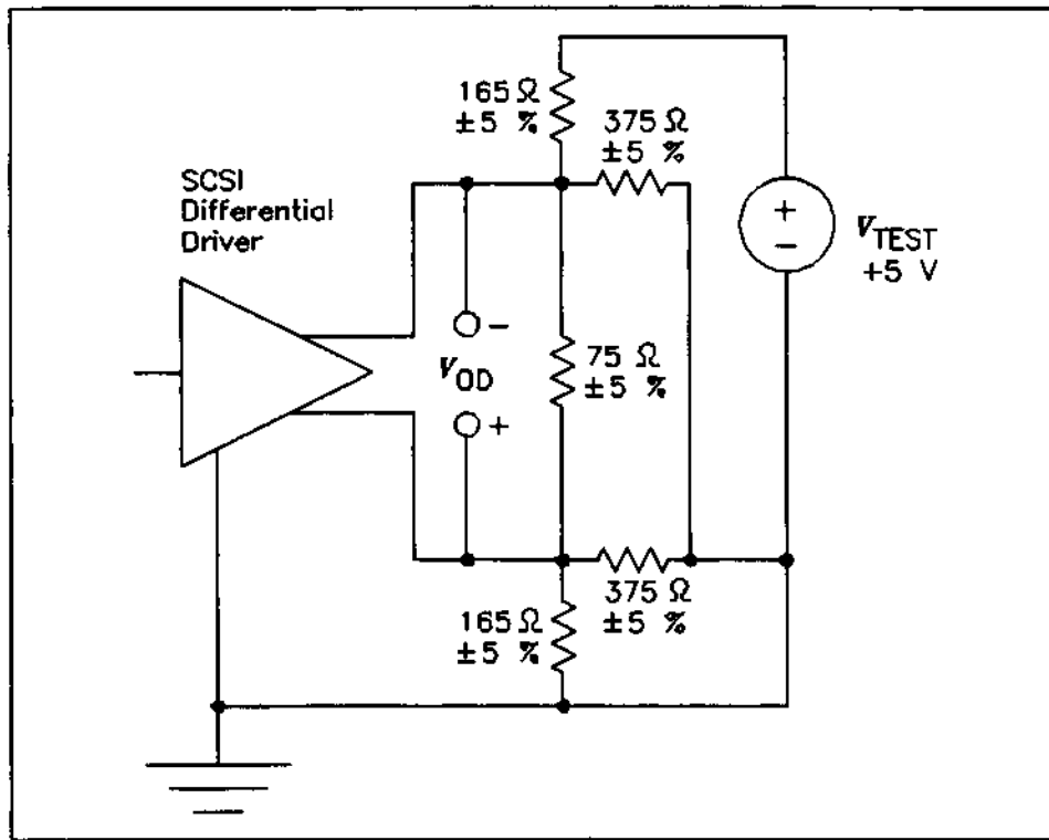
Figure 10 - Differential test circuit
