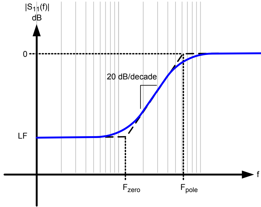
Figure A.4 — S-parameter return loss model plot
