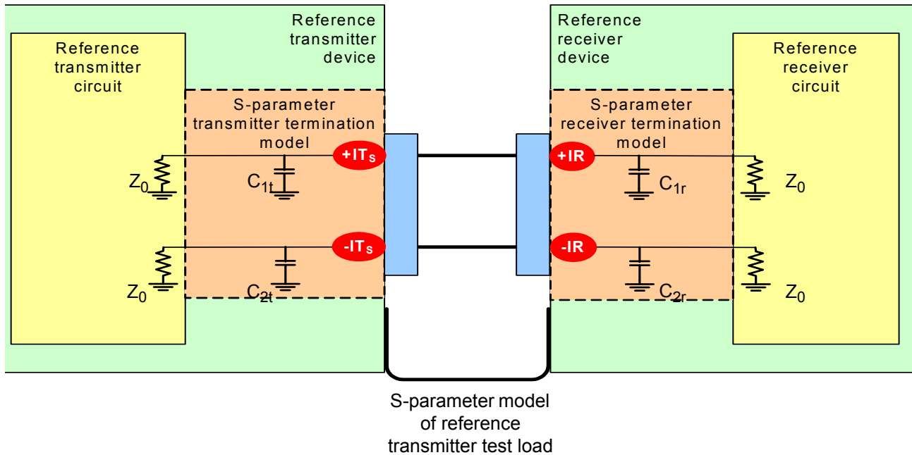
Figure A.1 — S-parameters modeling circuits for simulation
