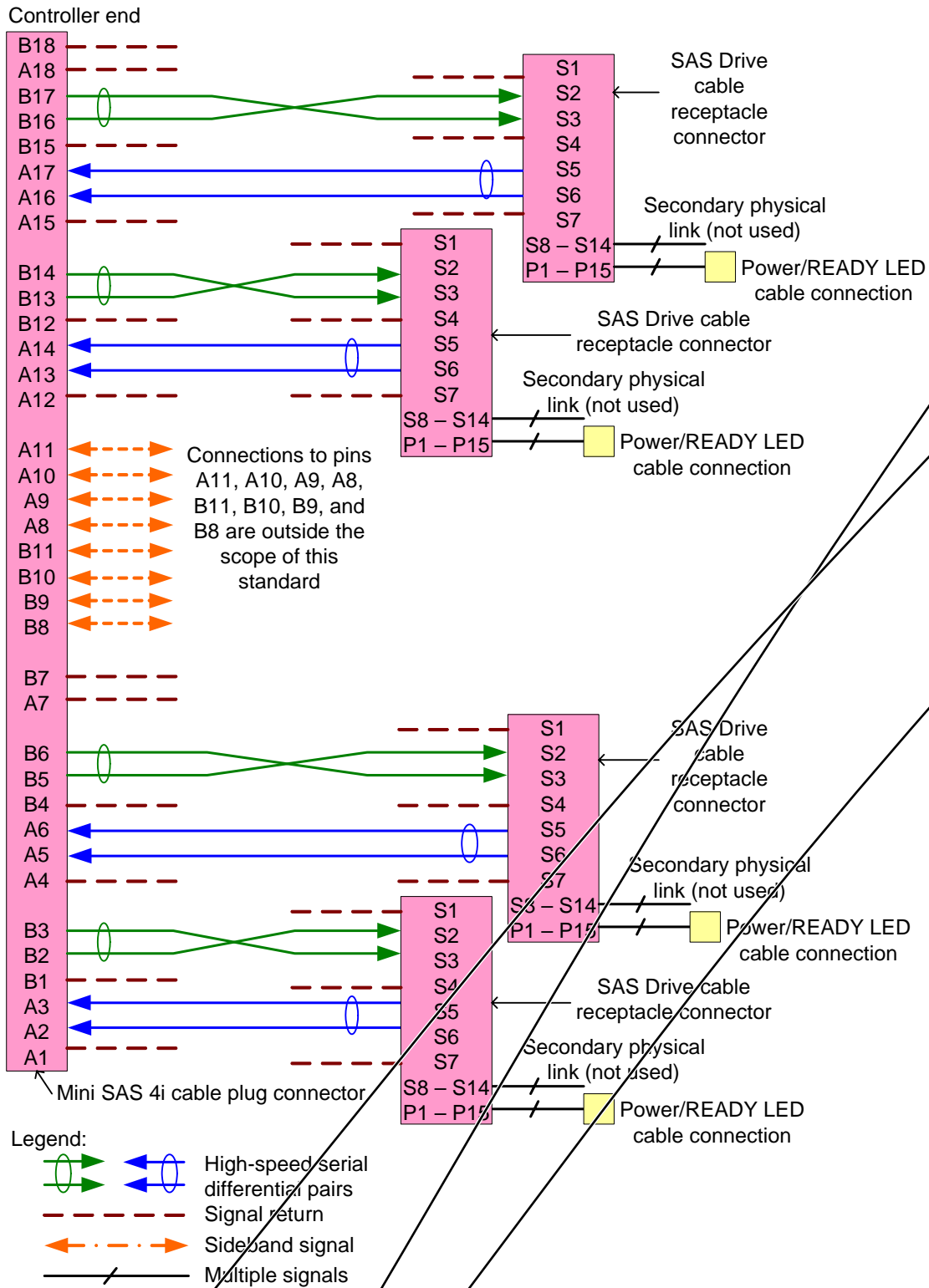
Figure 91 — SAS internal controller-based fanout cable assembly - Mini SAS 4i
