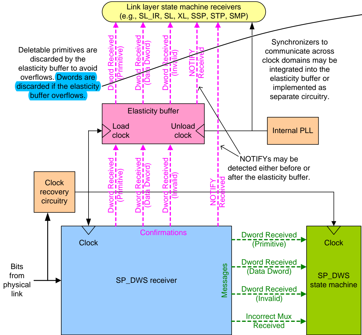
Figure 168 — Elasticity buffer
