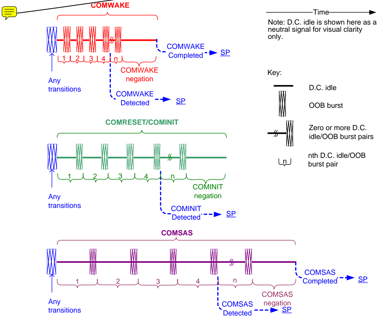
Figure 137 — OOB signal detection
