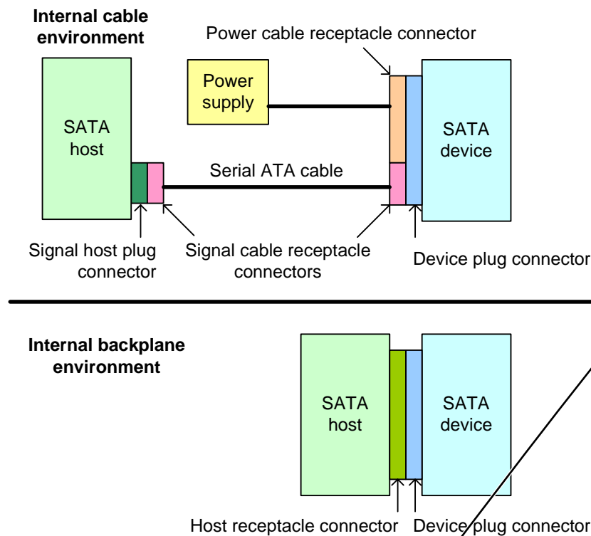
Figure 58 — SATA connectors and cables
