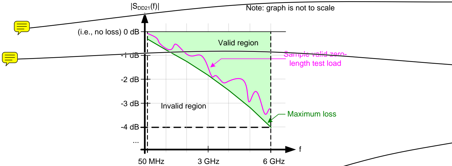
Figure 107 — Zero-length test load S_{DD21}
