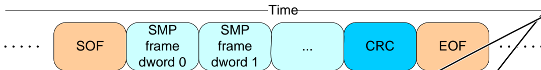
Figure 203 — SMP frame transmission
