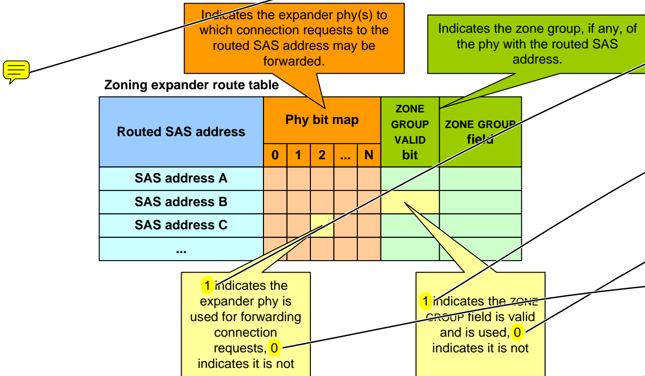
Figure 56 — Zoning expander route table
