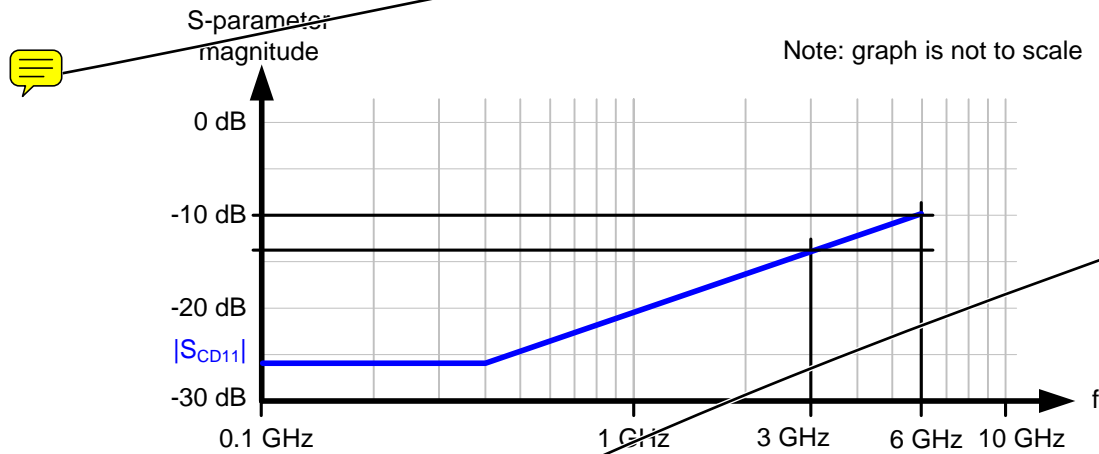
Figure 129 — Receiver device S_{CD11} limits
