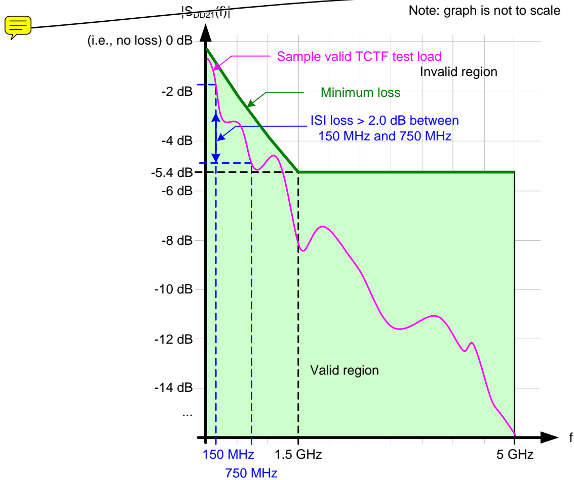
Figure 111 — TCTF test load S_{DD21} and ISI loss requirements at IT at 1.5 Gbps
