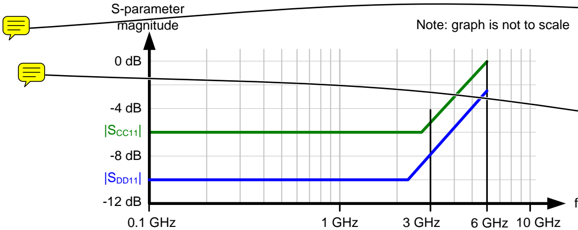
Figure 128 — Receiver device S_{CC11} and S_{DD11} limits
