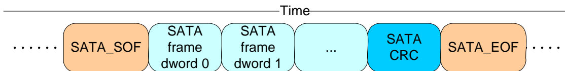
Figure 196 — STP frame transmission
