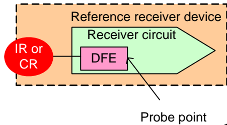
Figure 130 — Reference receiver device
