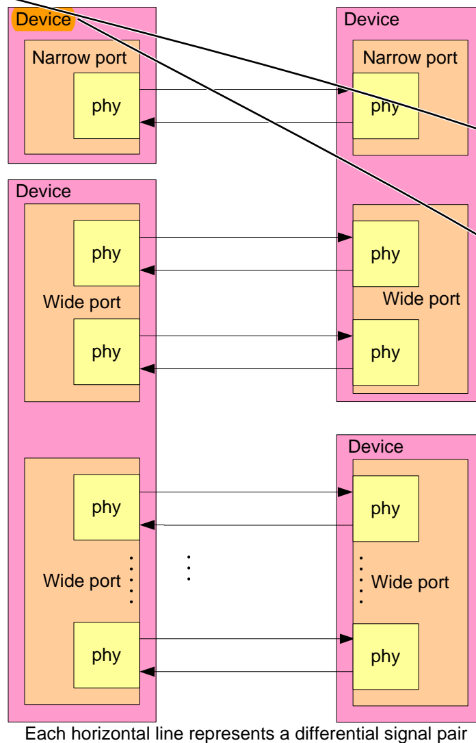
Figure 18 — SAS devices
