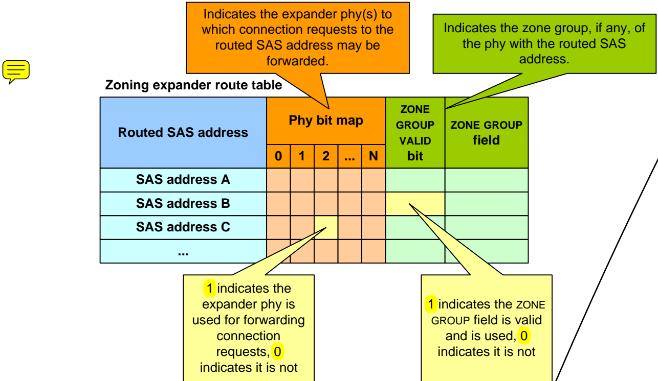
Figure 56 — Zoning expander route table
