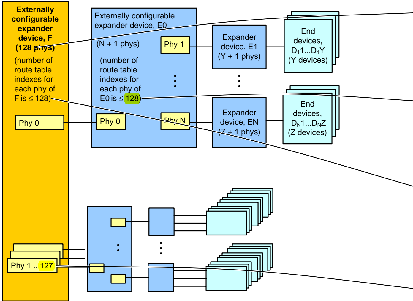
Figure 50 — Expander route index order example
