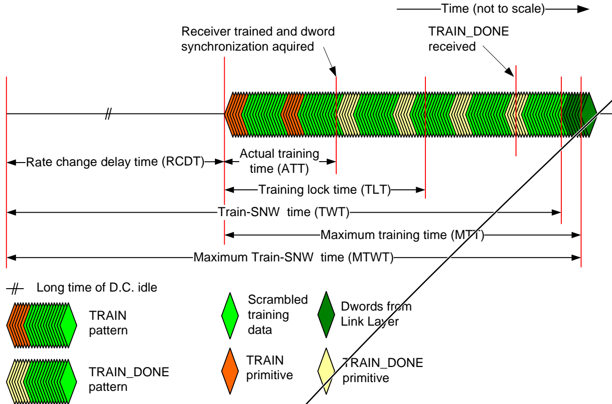
Figure 145 — Train-SNW
