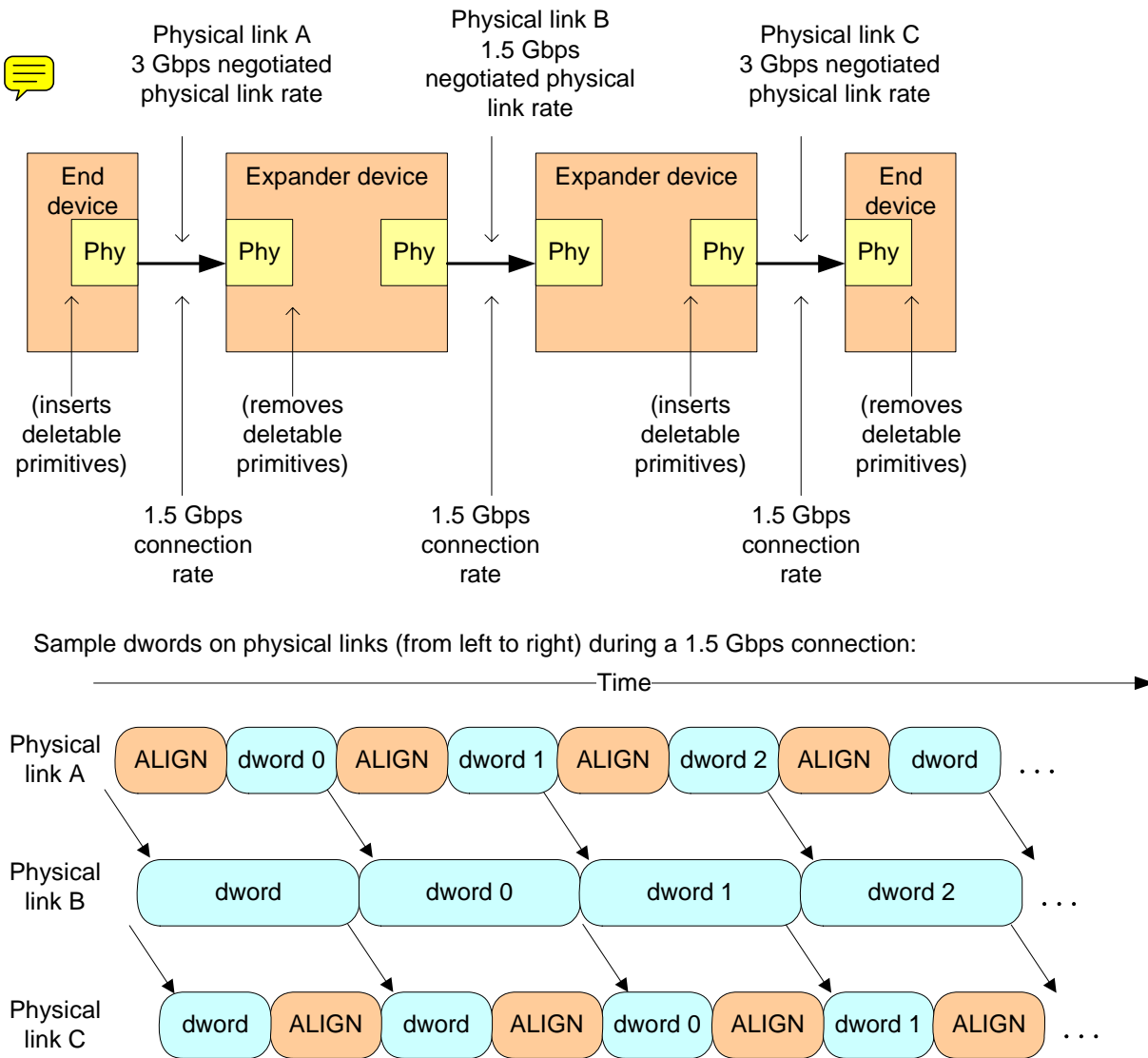
Figure 183 — Rate matching example
