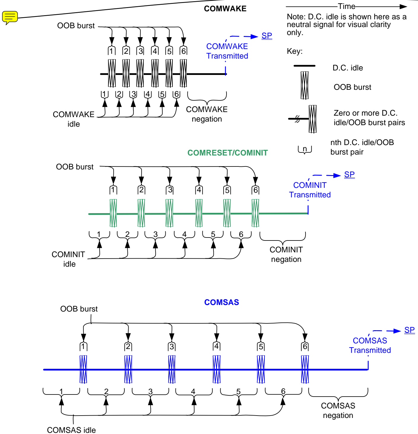
Figure 136 — OOB signal transmission
