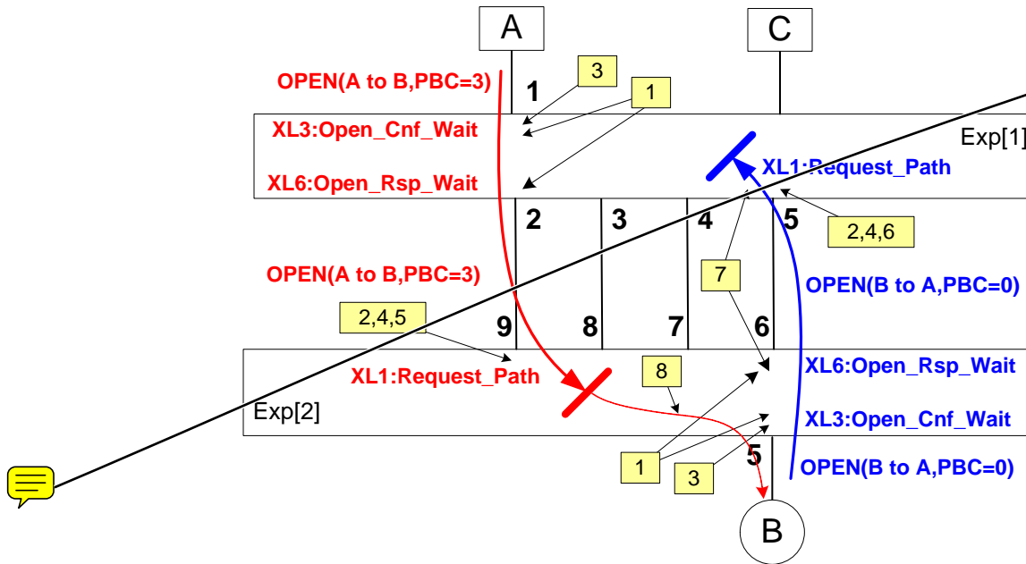
Figure J.19 — Partial pathway recovery
