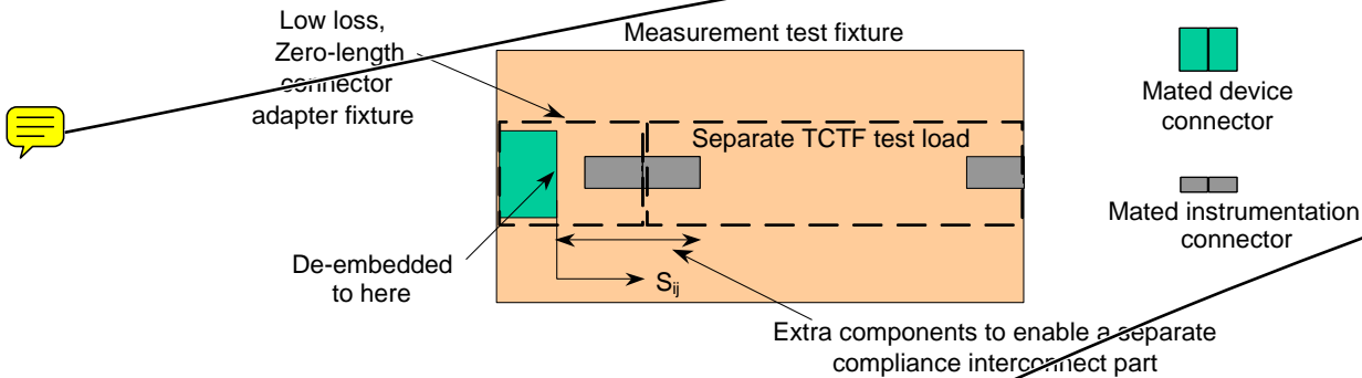
Figure B.6 — Transmitter device signal output measurement test fixture details
