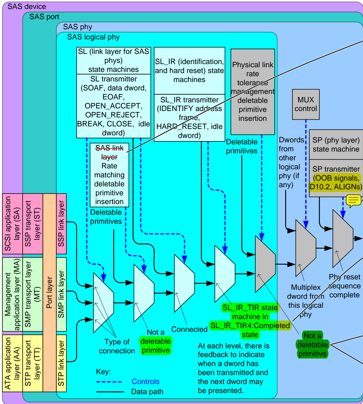
Figure 31 — Transmit data path in a SAS phy
