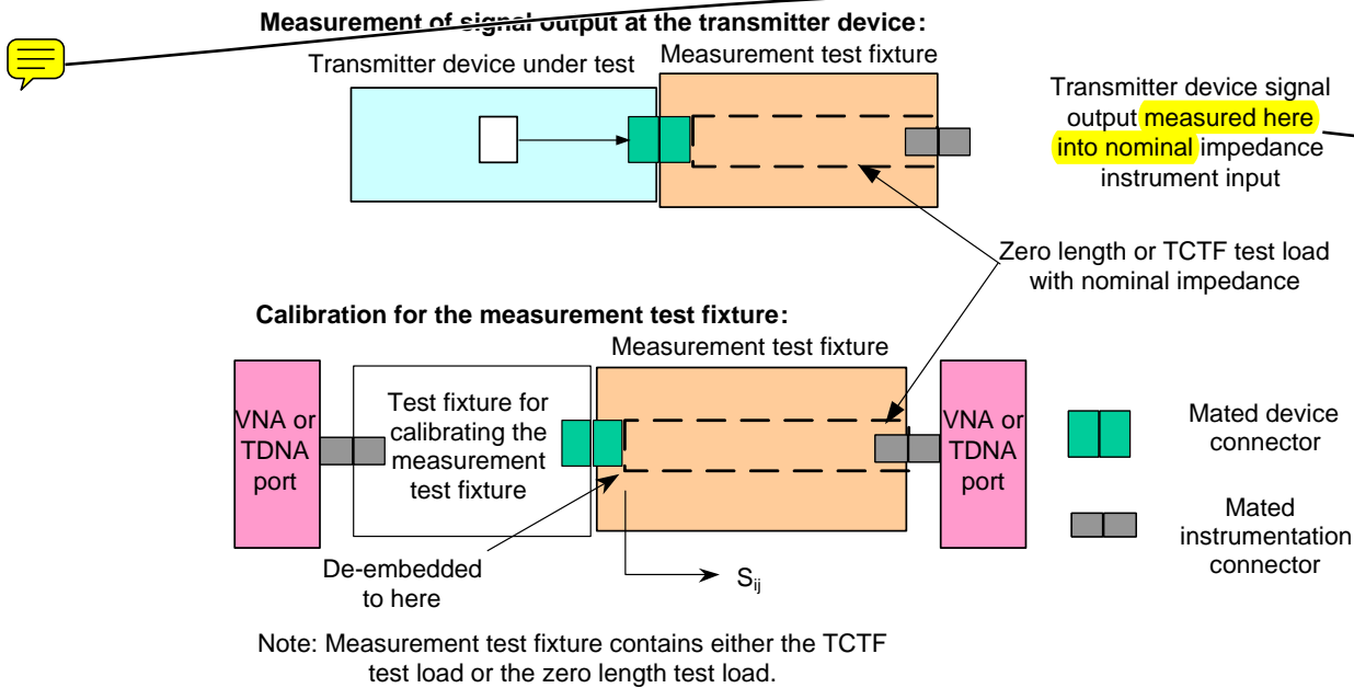
Figure B.5 — Measurement conditions for signal output at the transmitter device
