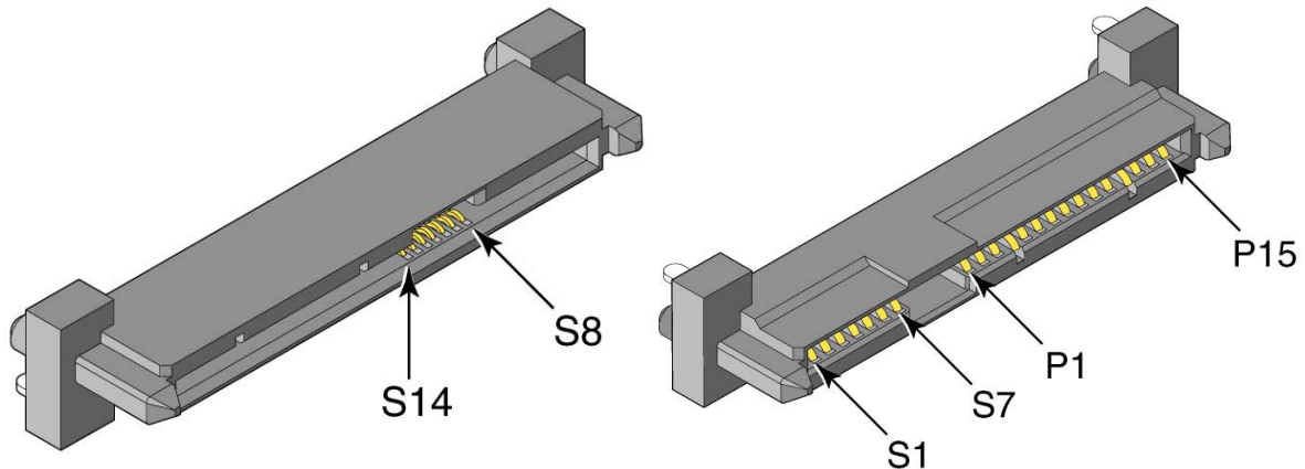
Figure 69 — SAS Drive backplane receptacle connector
