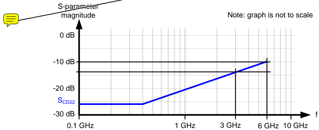
Figure 126 — Transmitter device S_{CD22} limits
