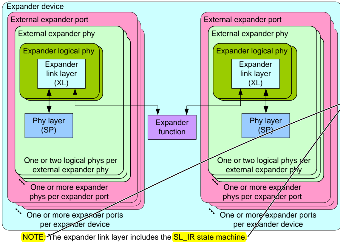
Figure 30 — State machines for expander devices
