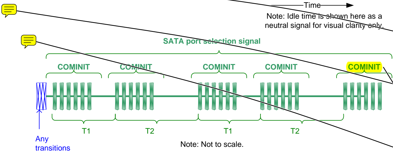
Figure 138 — SATA port selection signal
