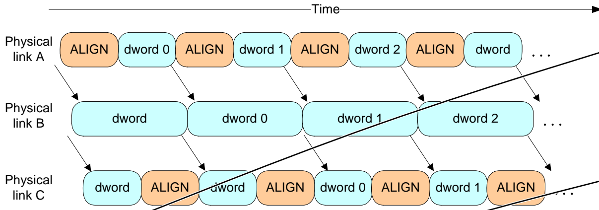
Figure 183 — Rate matching example
