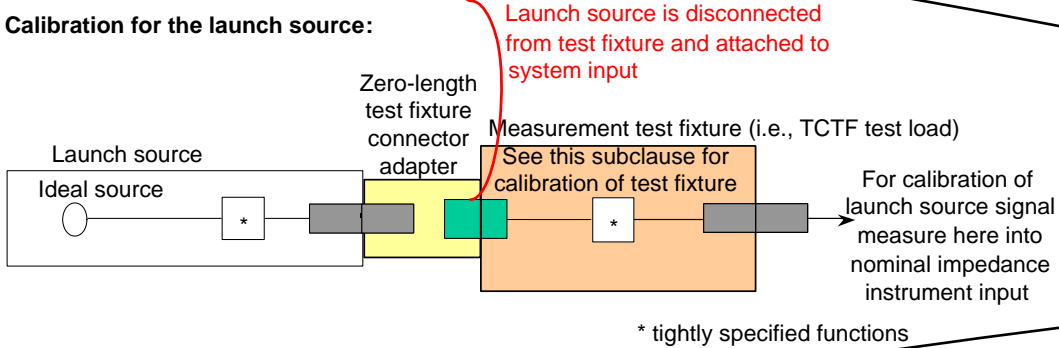
Figure B.7 — Measurement conditions for signal tolerance at the transmitter device
