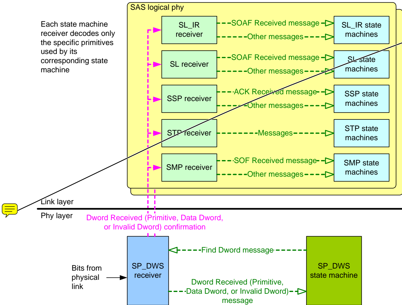
Figure 36 — Receive data path in a SAS phy
