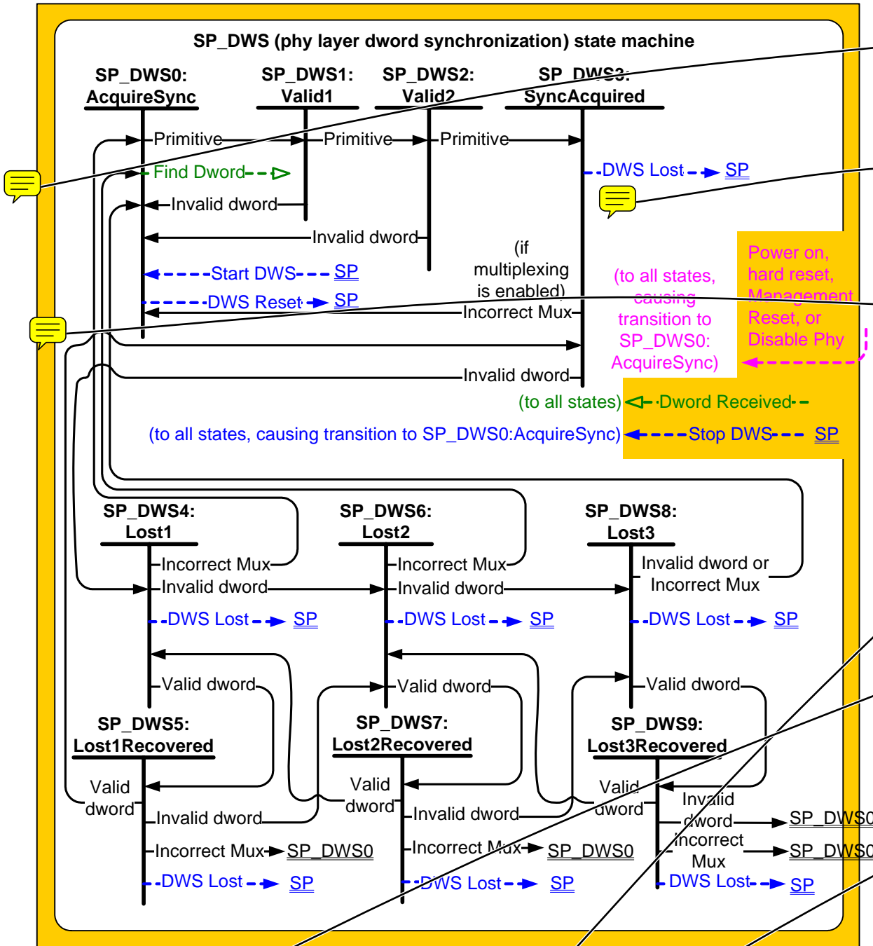
Figure 160 — SP_DWS (phy layer dword synchronization) state machine
