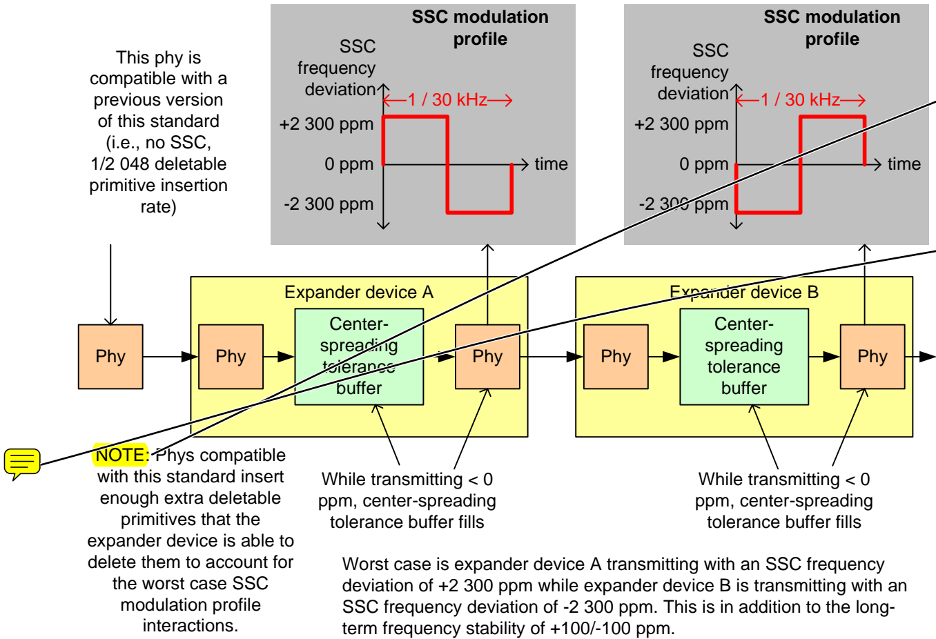
Figure 133 — Center-spreading tolerance buffer
