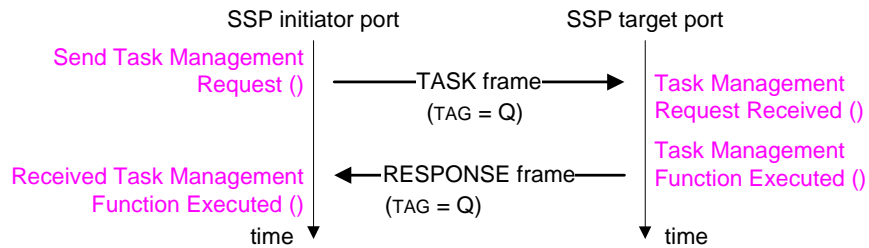
Figure 210 — Task management function sequence of SSP frames
