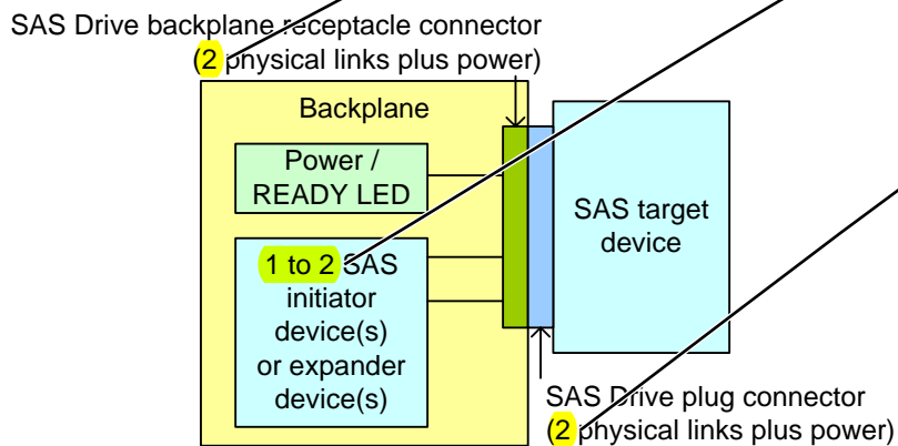
Figure 60 — SAS Drive backplane environment
