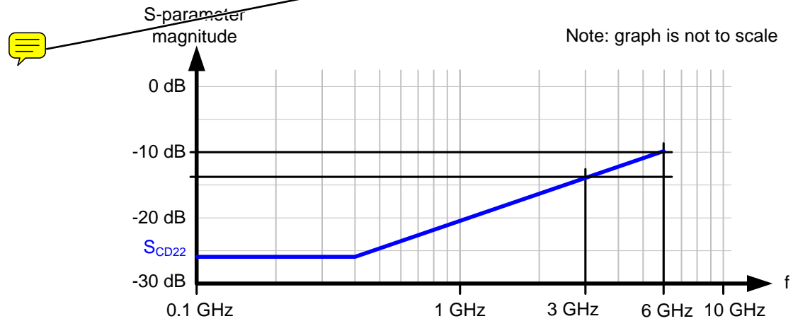
Figure 126 — Transmitter device S_{CD22} limits
