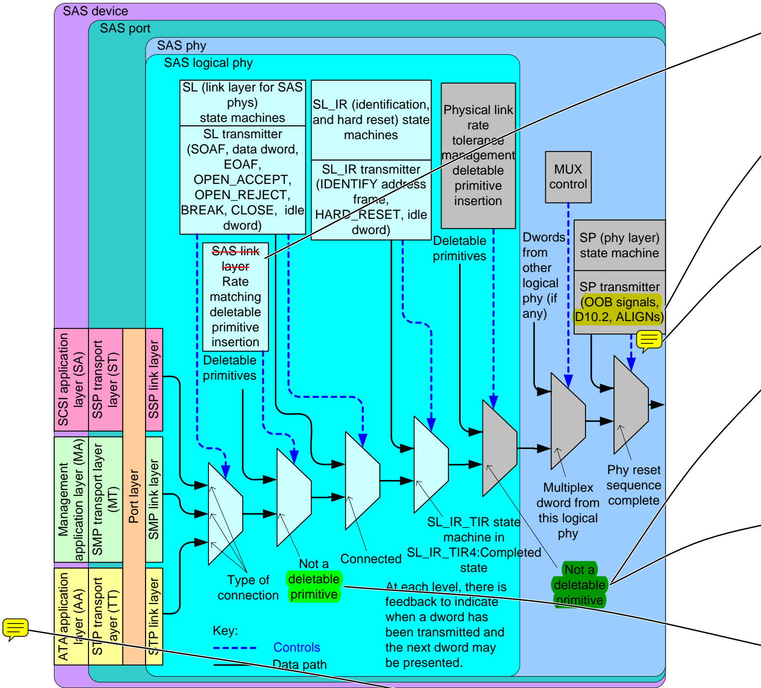
Figure 31 — Transmit data path in a SAS phy
