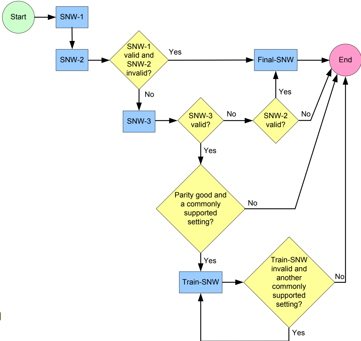
Figure 146 — SAS speed negotiation sequence SNW flowchart
