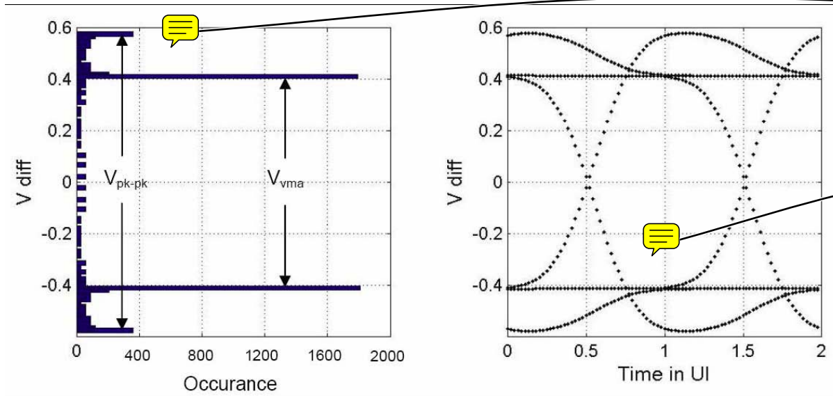
Figure 127 — Transmitter equalization measurement
