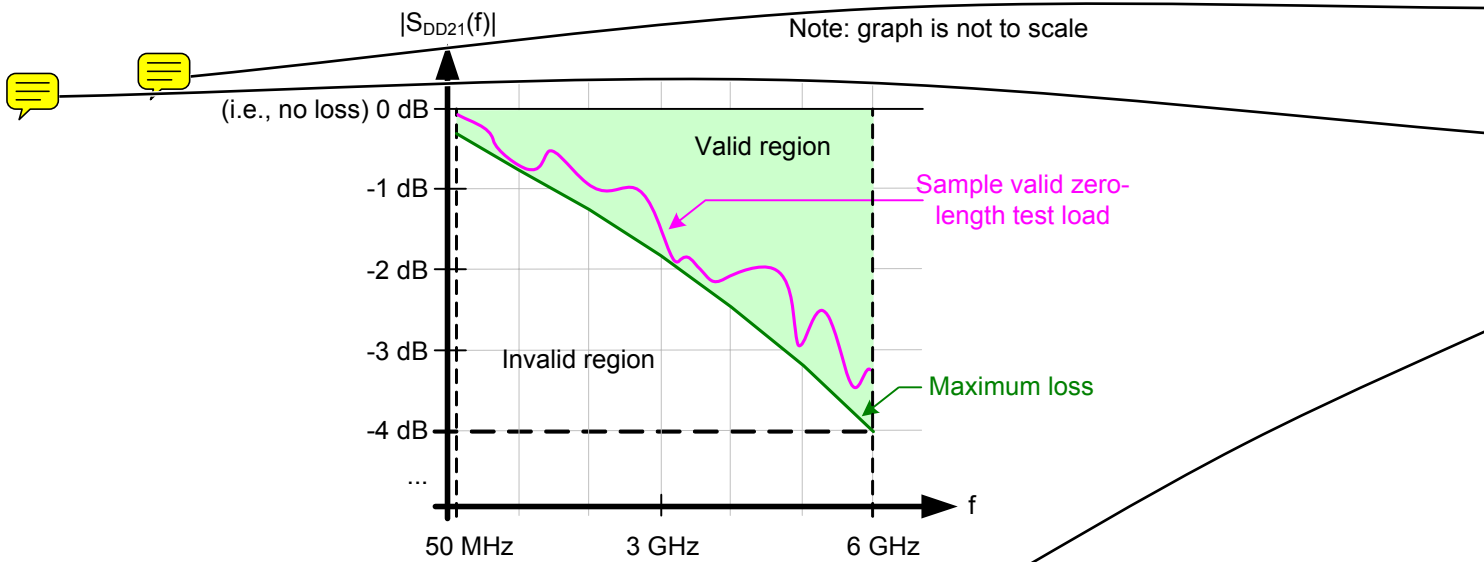
Figure 107 — Zero-length test load S_{DD21}
