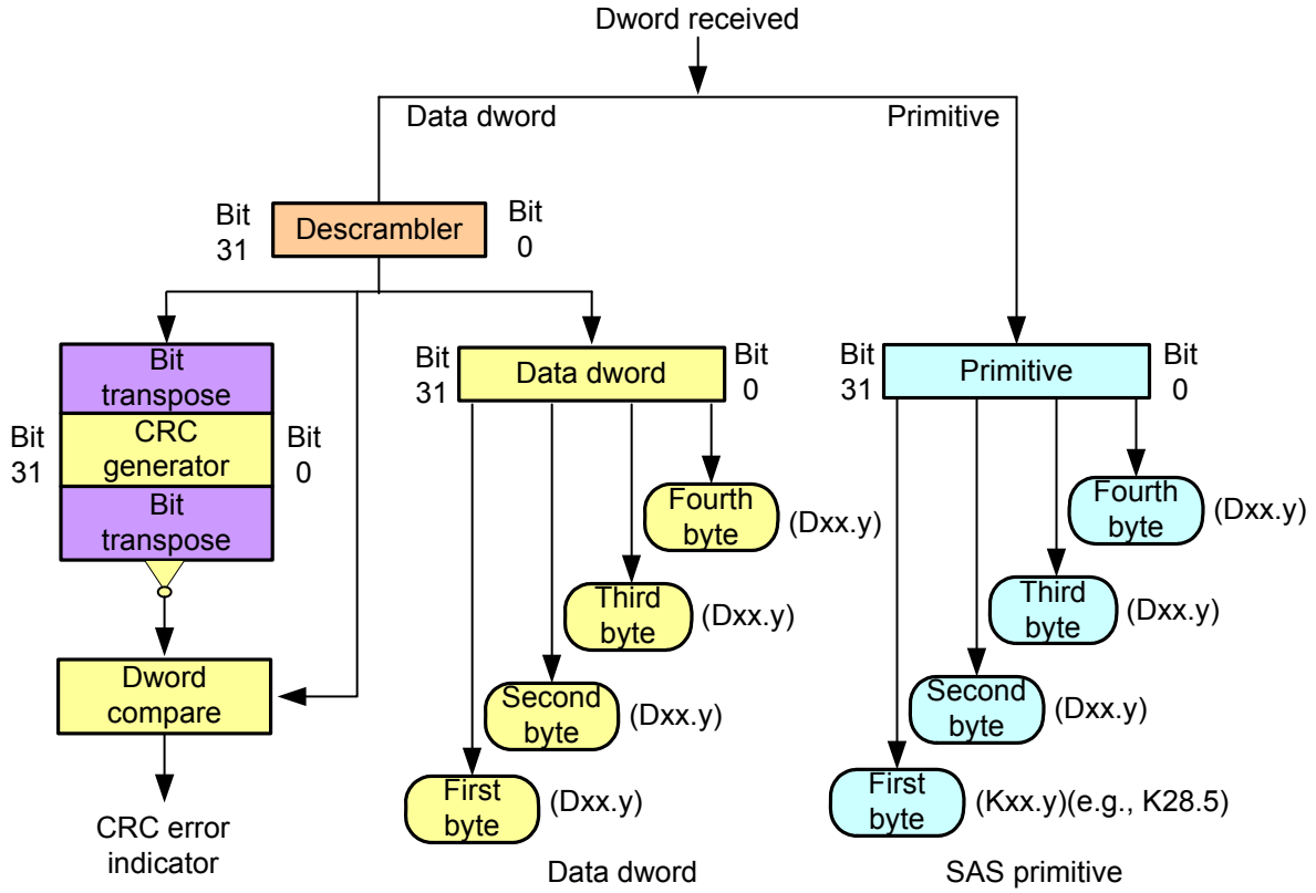
Figure 172 — Receive path bit ordering
