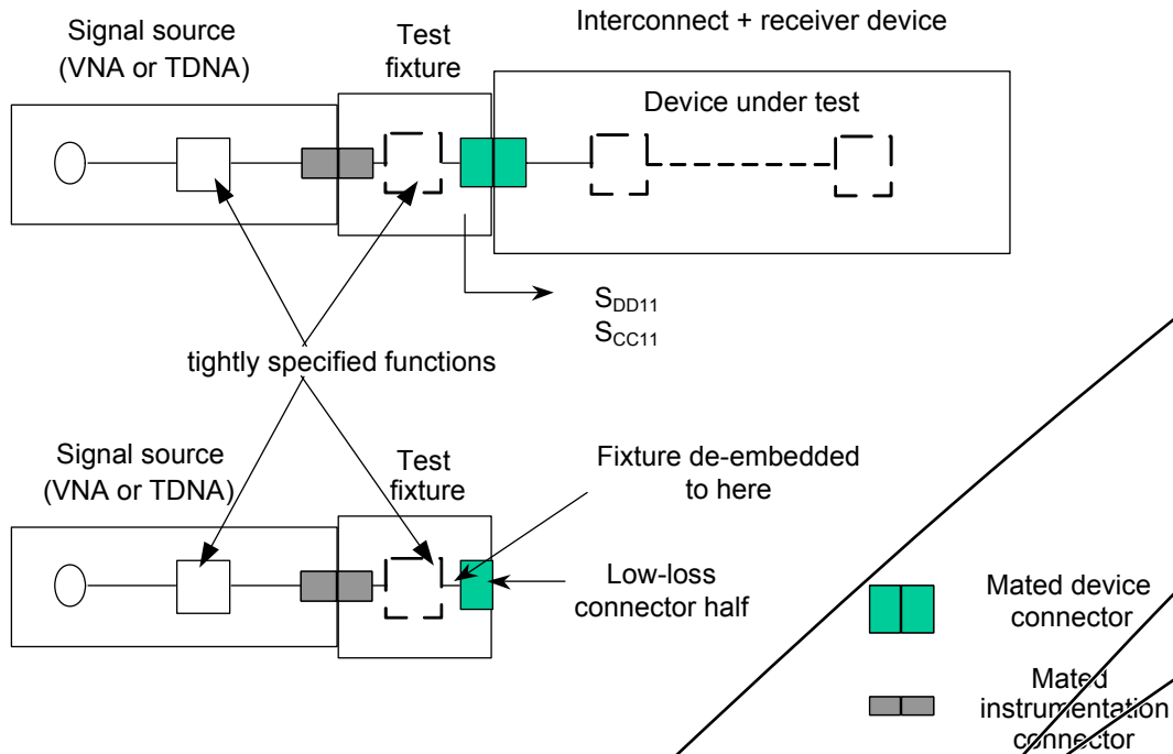
Figure B.17 — Measurement conditions for S_{11} at IT or CR
