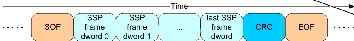
Figure 189 — SSP frame transmission
