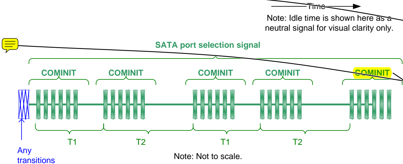
Figure 138 — SATA port selection signal
