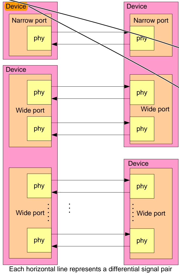
Figure 18 — SAS devices
