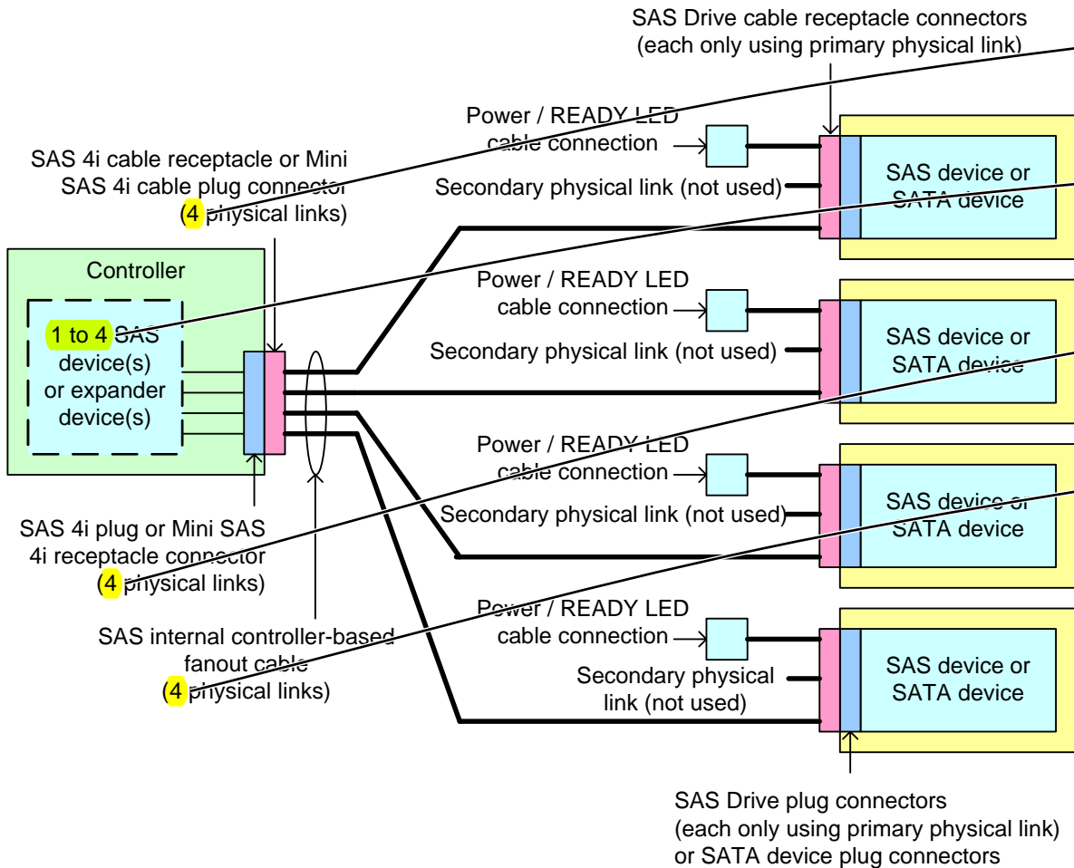
Figure 64 — SAS internal controller-based fanout cable environment
