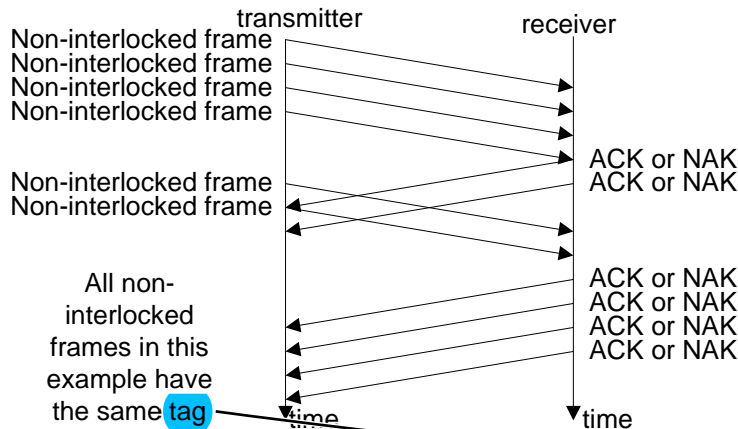
Figure 191 — Non-interlocked frames with the same tag
