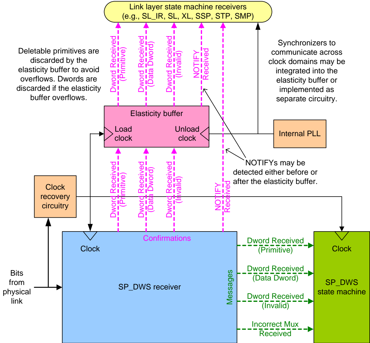
Figure 156 — Elasticity buffers
