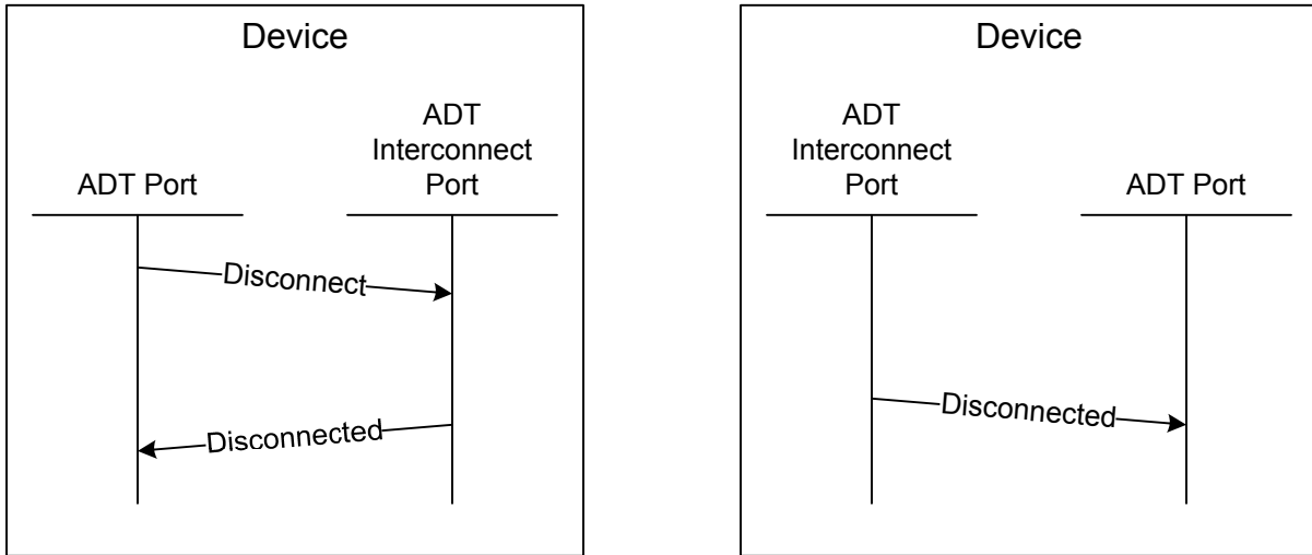
Figure 20 – Protocol services for closing a connection between ADT serial ports
