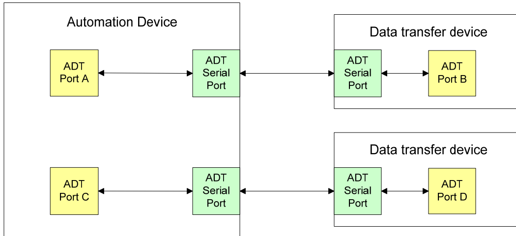
Figure 8 – ADT serial port example
