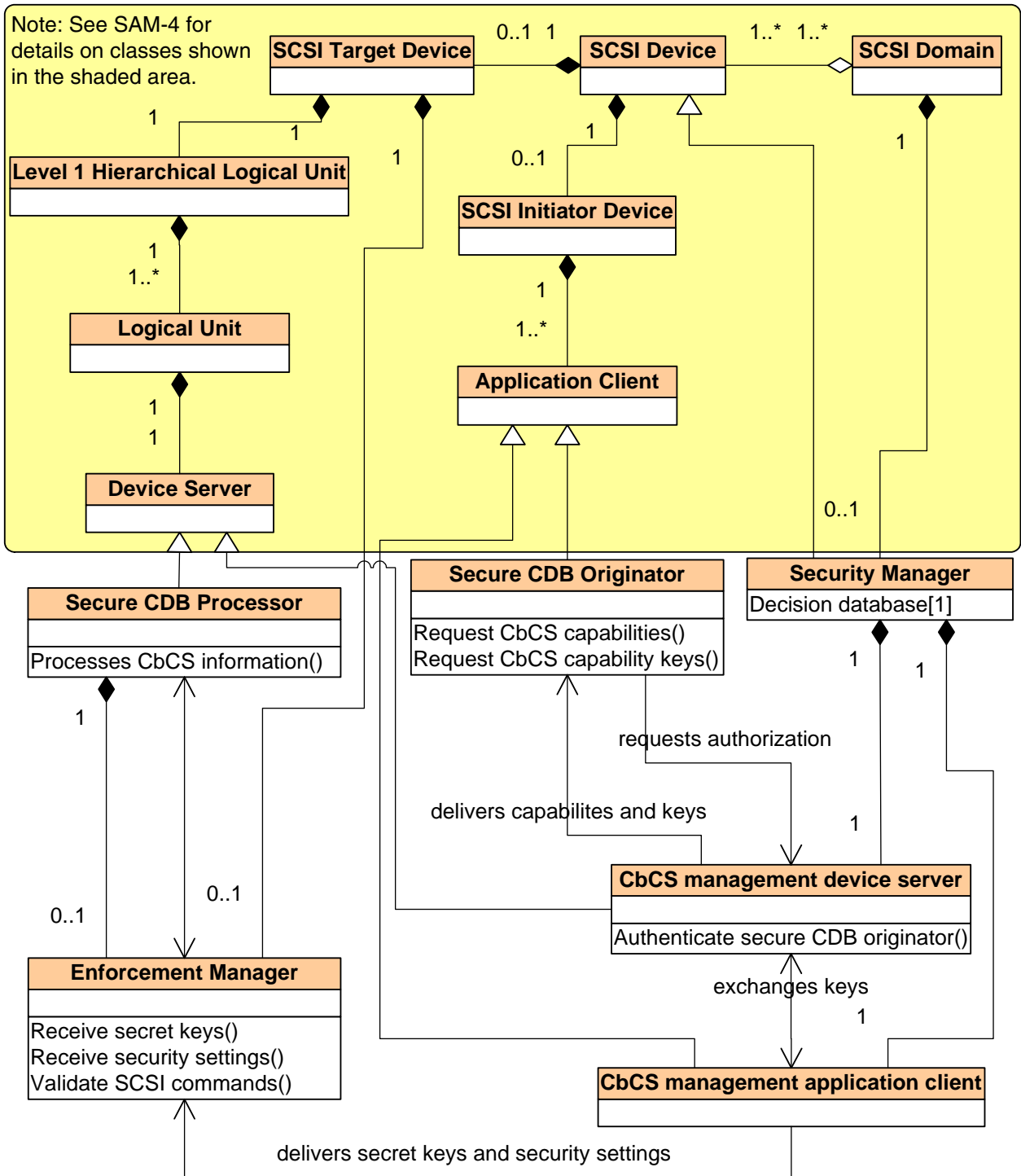
Figure 1 — CbSC class diagram
