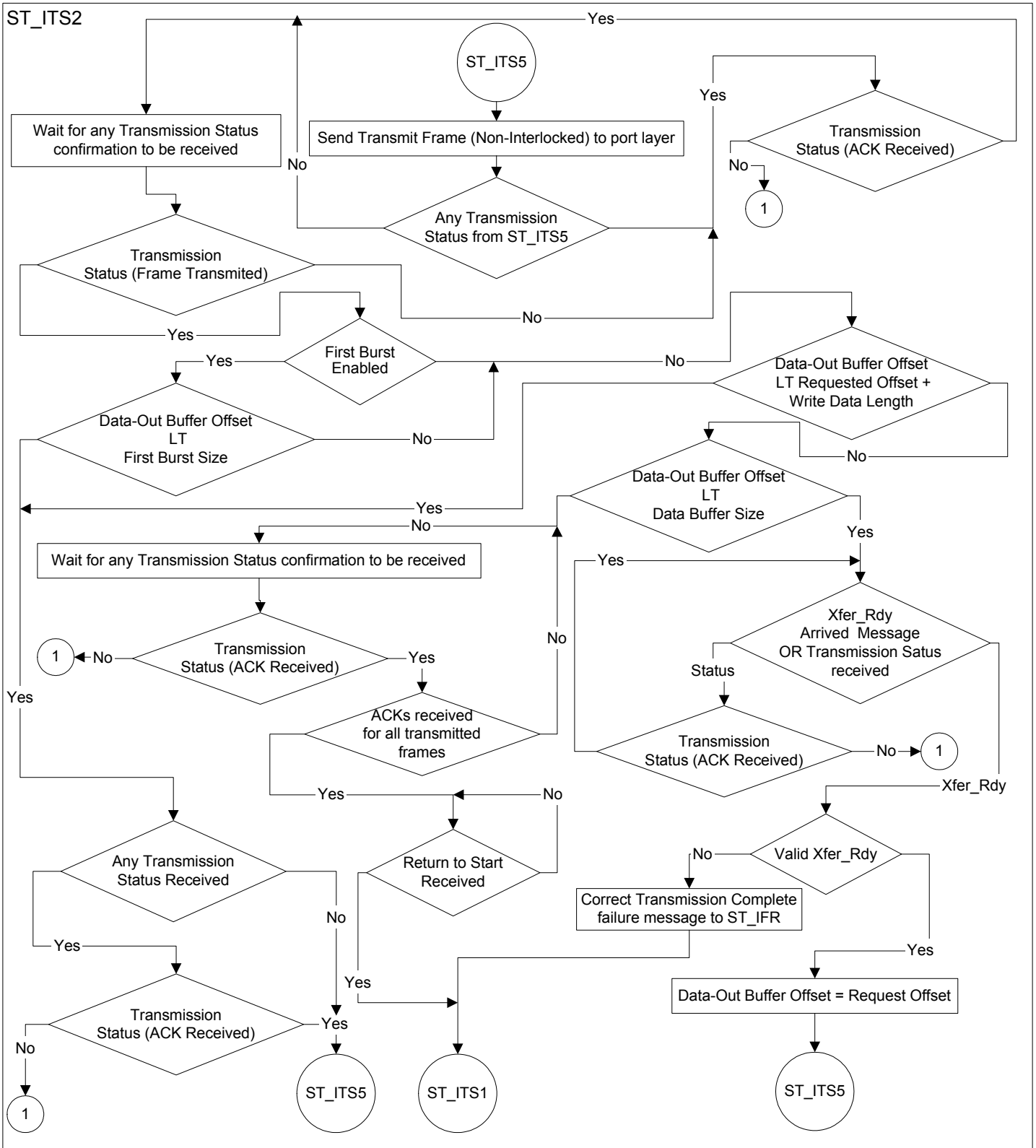
Figure 2 — Representation of transport layer (i.e., ST_ITS2) write data operation (part 1 of 2)
