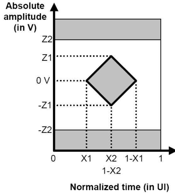
Figure 115 — Receiver device eye mask
