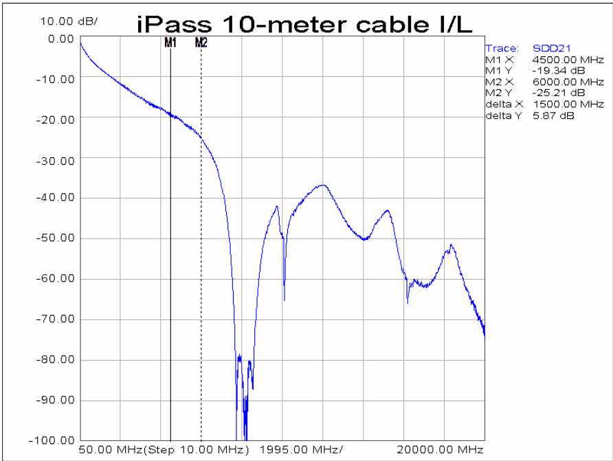
Figure 2. Differential cable insertion loss
