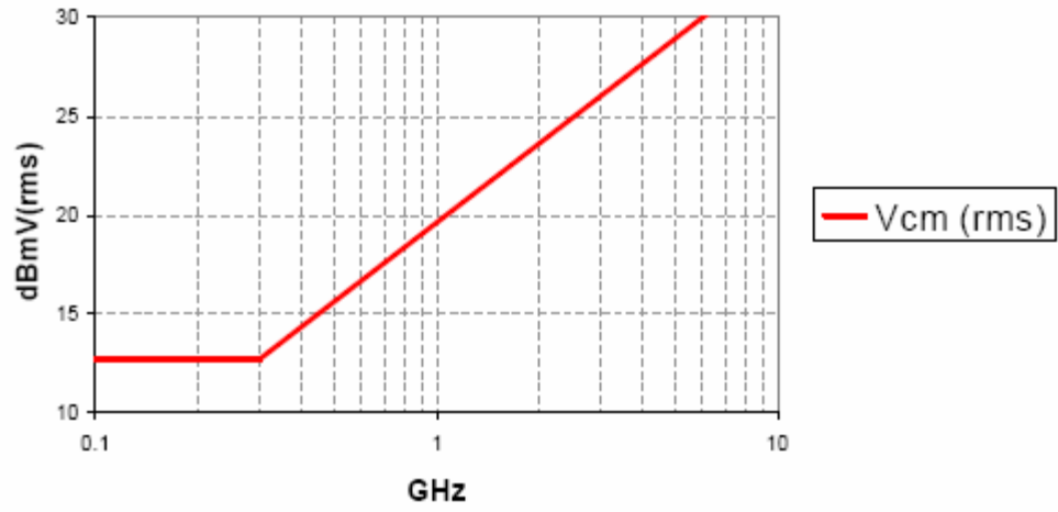
Transmitter device common mode voltage limit
