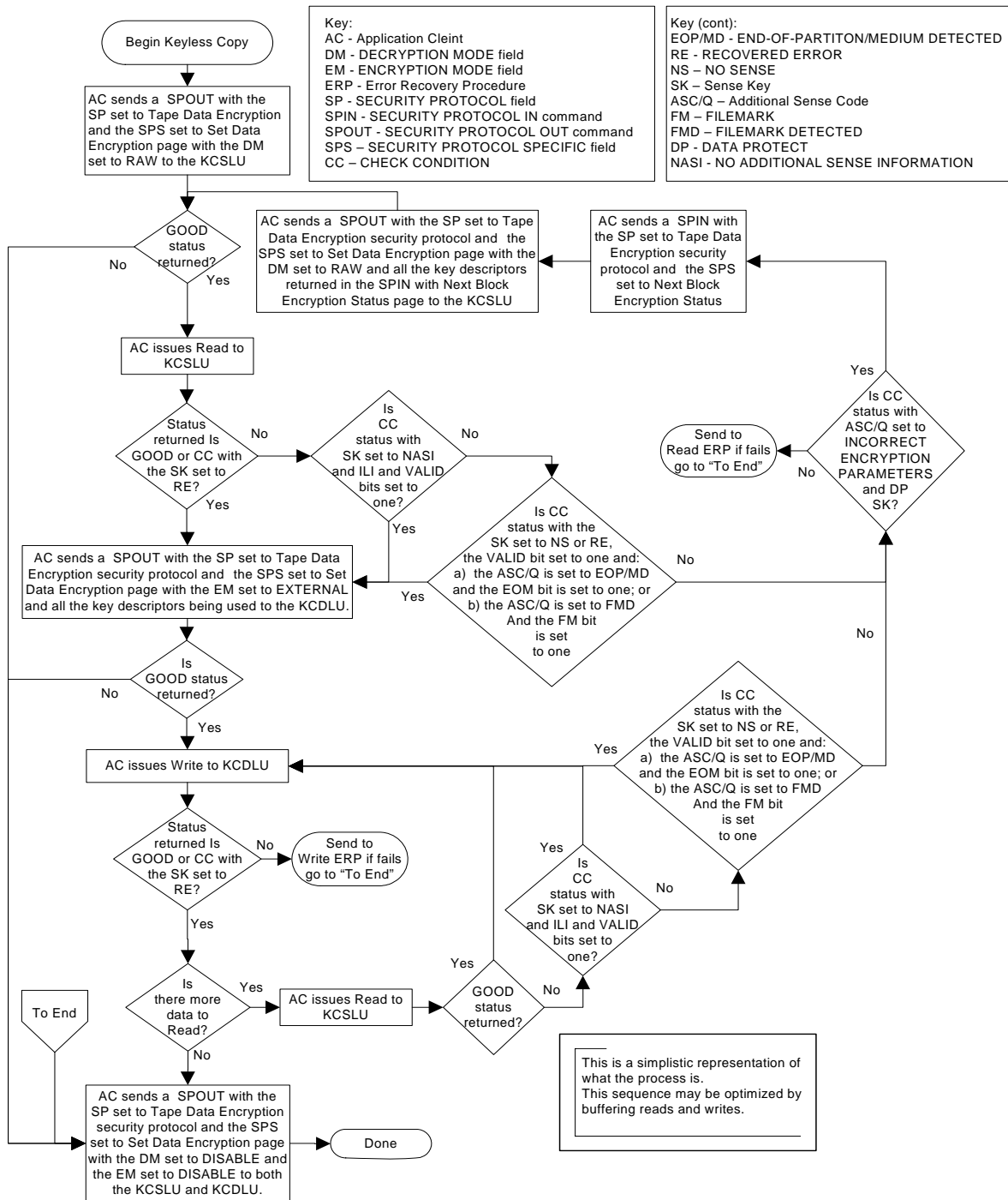
FIGURE 1. Flowchart describing a keyless copy operation
