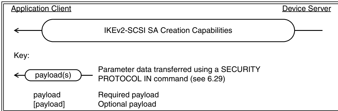
Figure x1 — IKEv2-SCSI Device Server Capabilities step
