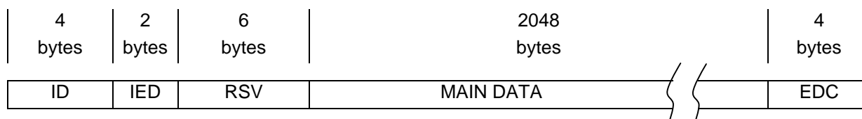
Figure 2 – Logical Layout of a DVD+RW Data Sector
