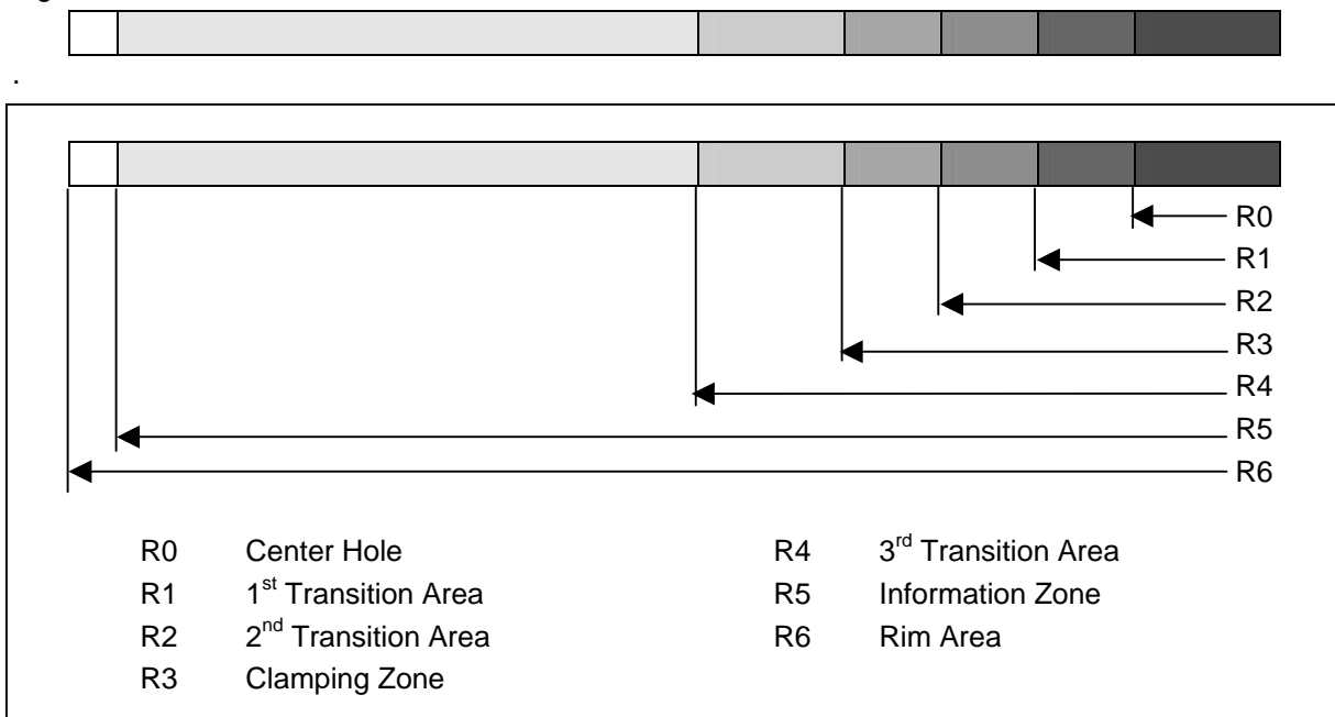
Figure 1 – The Zones of a DVD+RW Medium
