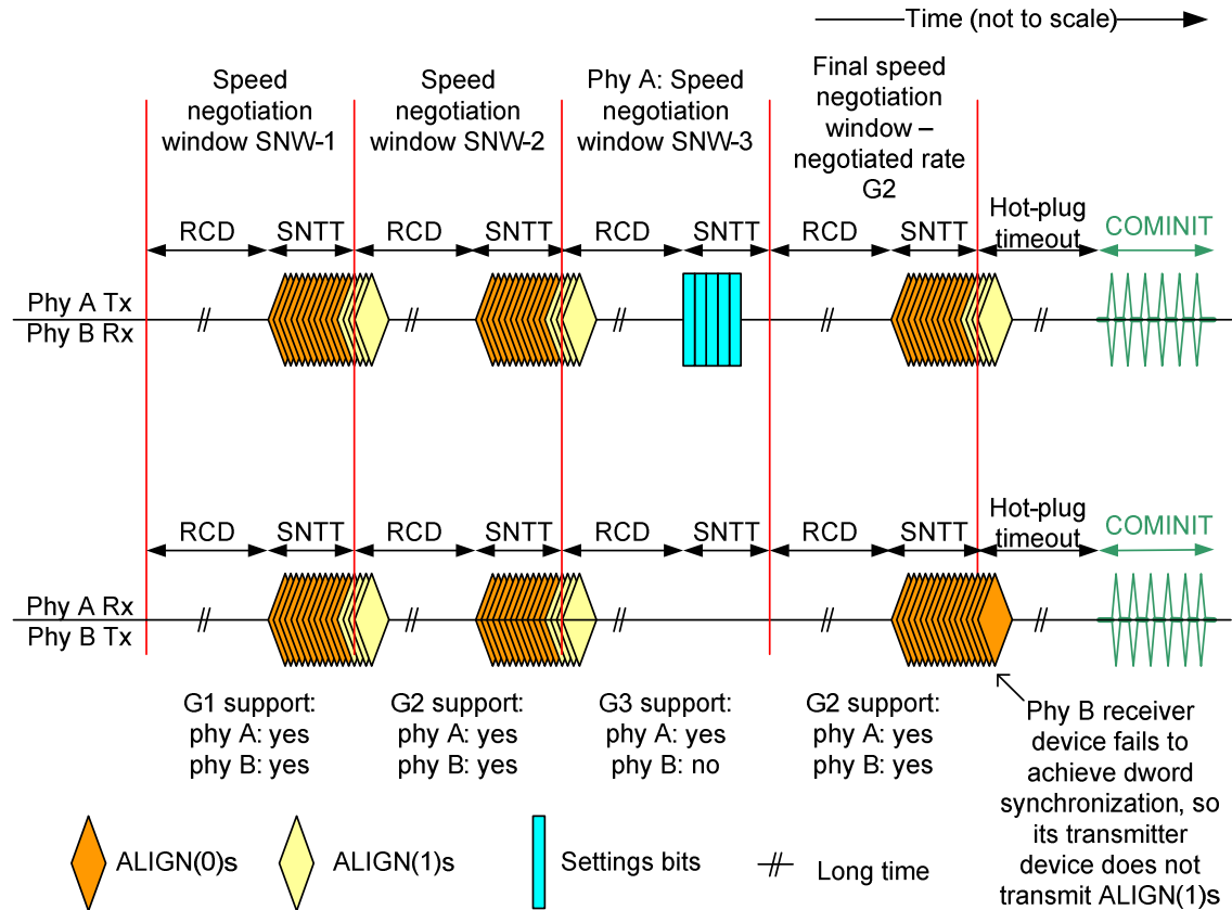
Figure 126 — SAS Final-SNW phy reset problem
