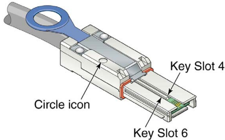
Figure 19 — Mini SAS 4x cable plug connector that attaches to an enclosure in port
