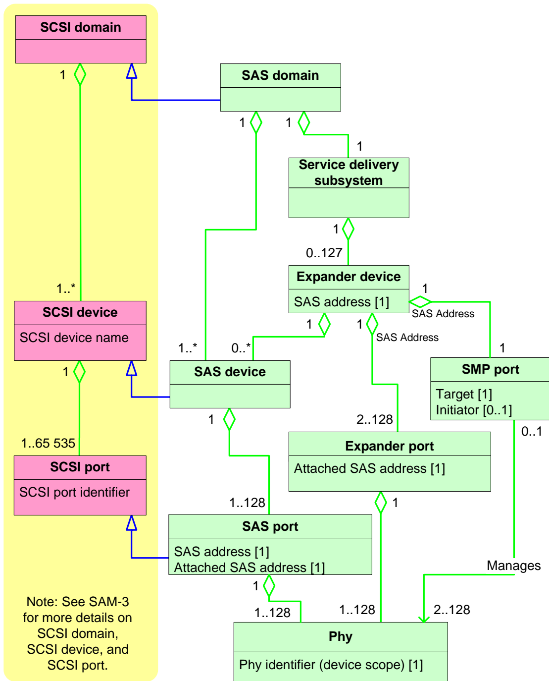
Figure 2 — SAS domain class diagram
