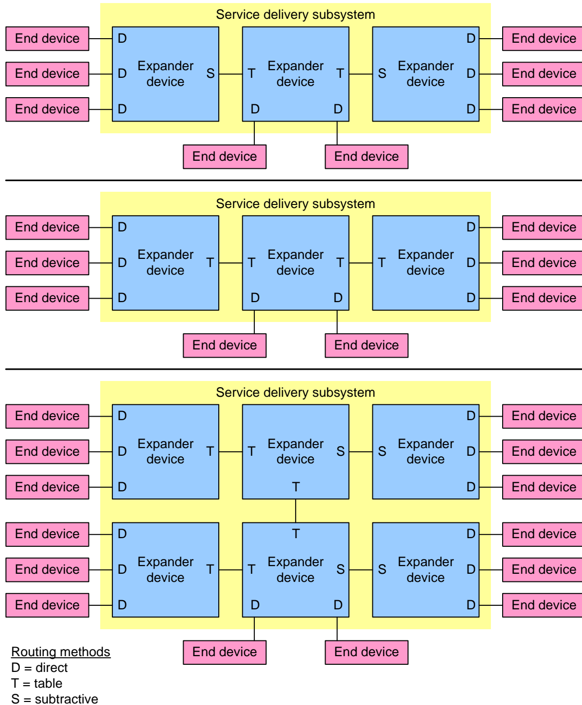
Figure 10 — Multiple expander device topologies
