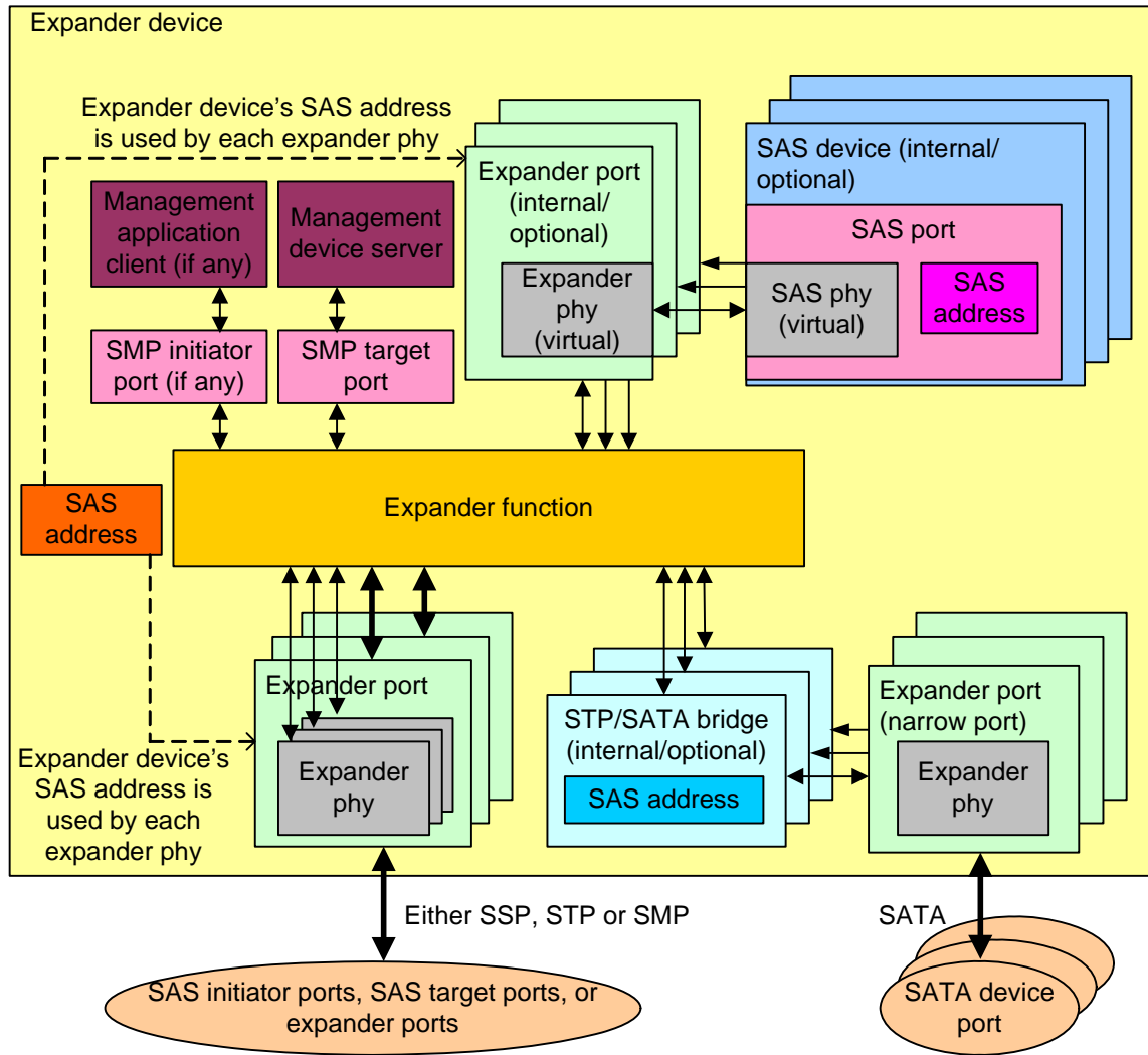
Figure 3 — Expander device
