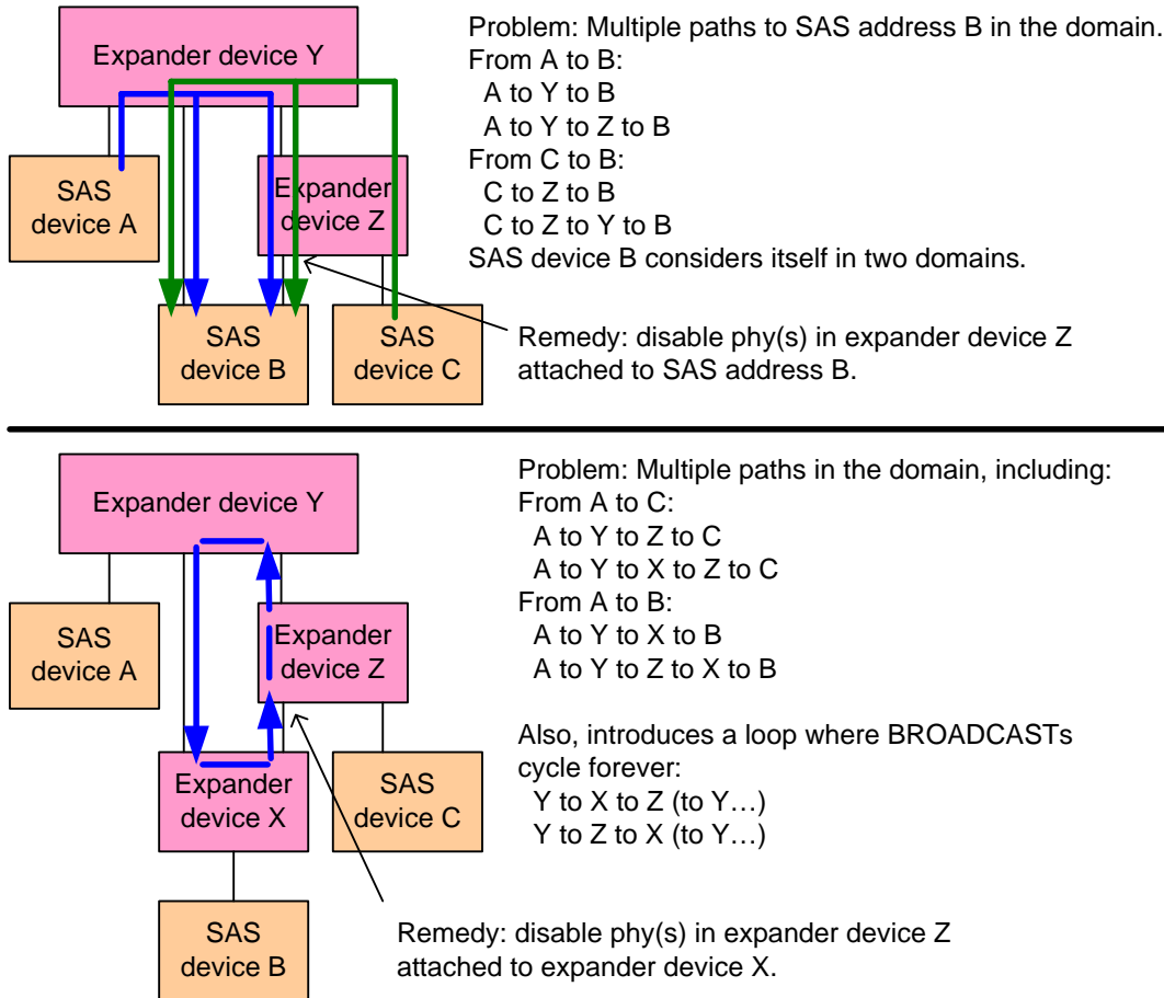
Figure 13 — Examples of invalid topologies
