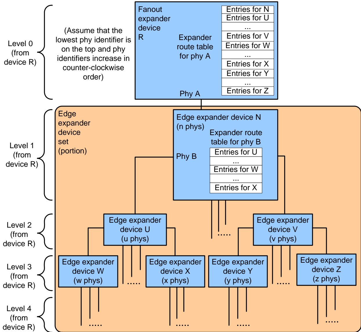
Figure 16 — Expander route index levels example with fanout expander device [TODO update]
