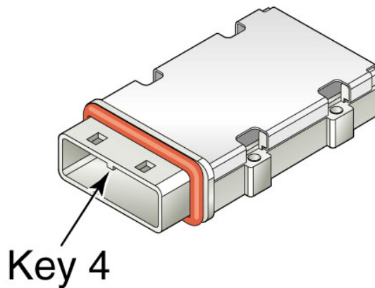
Figure 20 — Mini SAS 4x receptacle connector - end device or enclosure universal port
