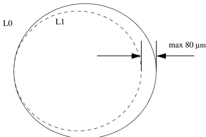
Figure 71 - Tolerance between L0 and L1
