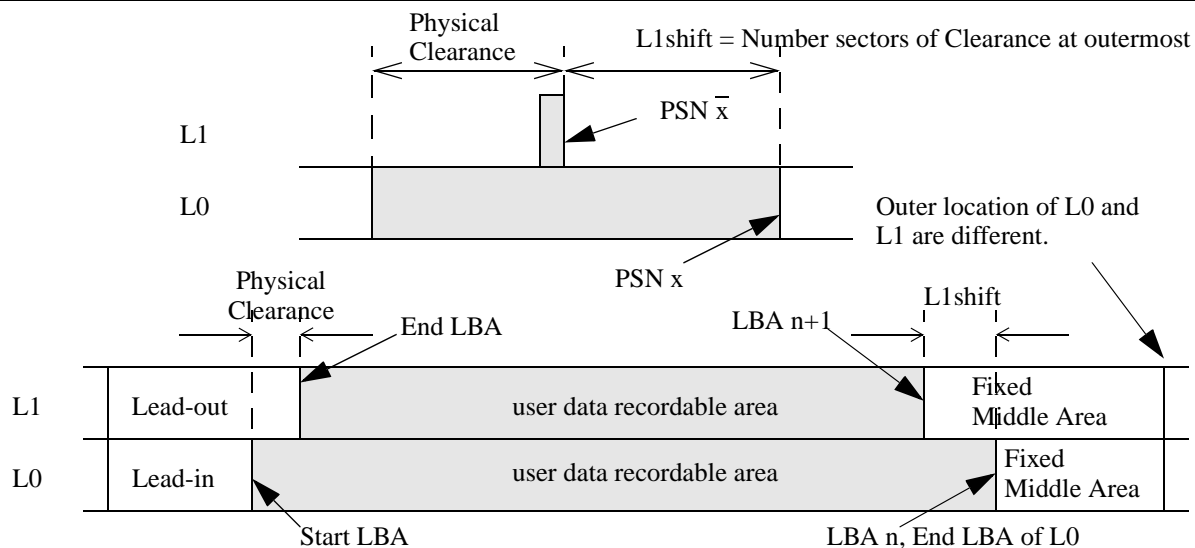
Figure 72 - Physical overview of Layers
