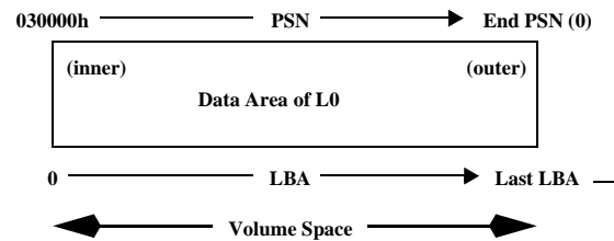
Figure 105 - Physical and logical layout of HD DVD-ROM Single Layer media
