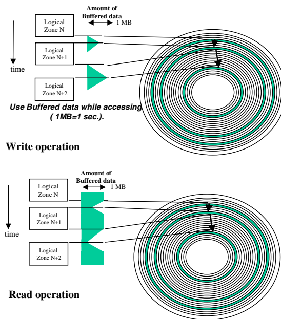
Figure 151 - Concept of seamless linking for AV capture/playback
