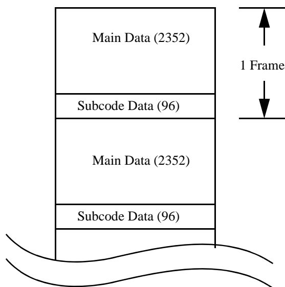
Figure 174 - Location of Sub-channel Data
