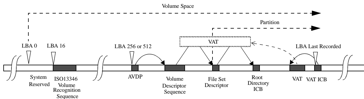
Figure 184 - Basic UDF Structure used on sequentially written media
