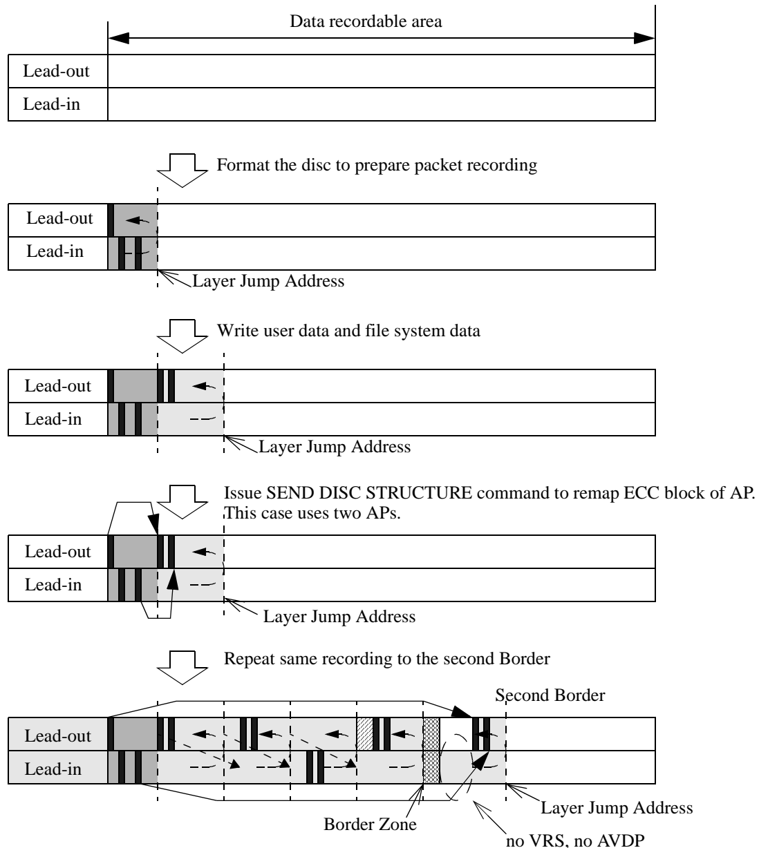
Figure 92 - Example sequence of Packet recording with remapping
