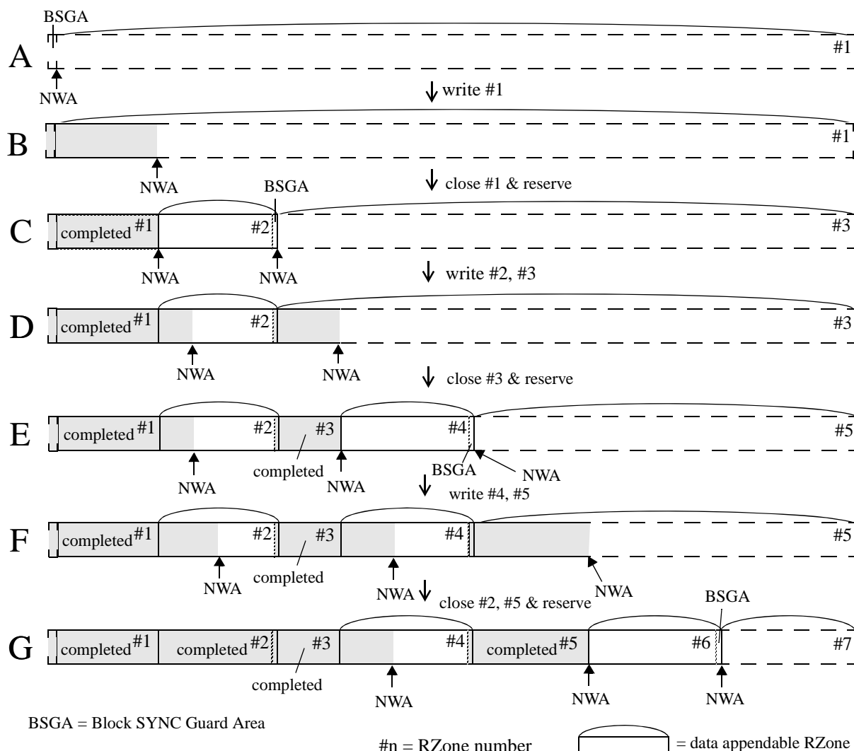
Figure 46 - Example of RZone reservation sequence
