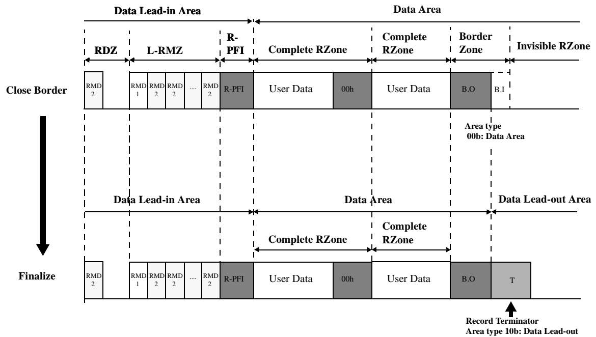
Figure 135 - Disc Final Closure with Terminator
