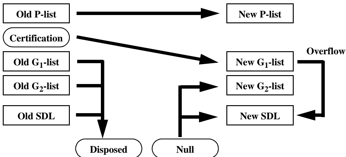
Figure 30 - Formatting Type 1 - Slow Initialization
