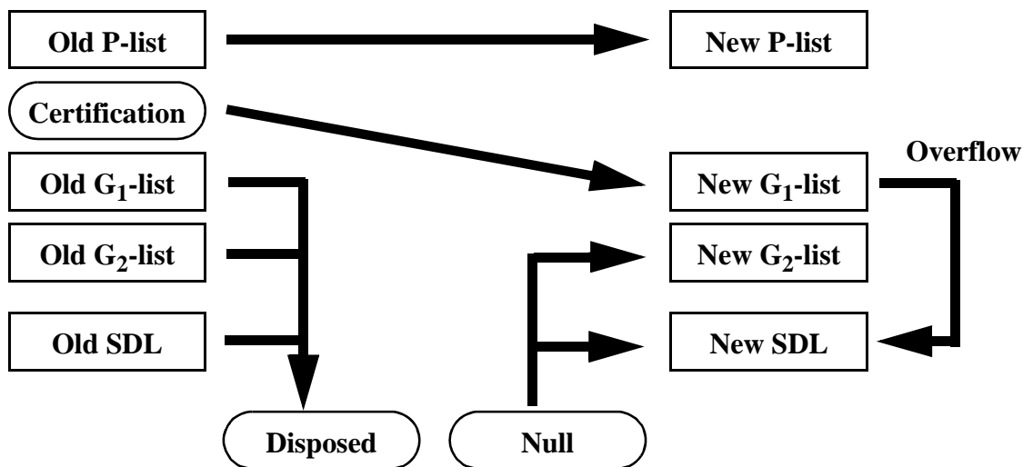
Figure 145 - Formatting Type 1 - Slow Initialization
