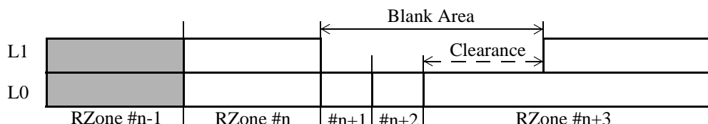
Figure 74 - Small Reserved RZone
