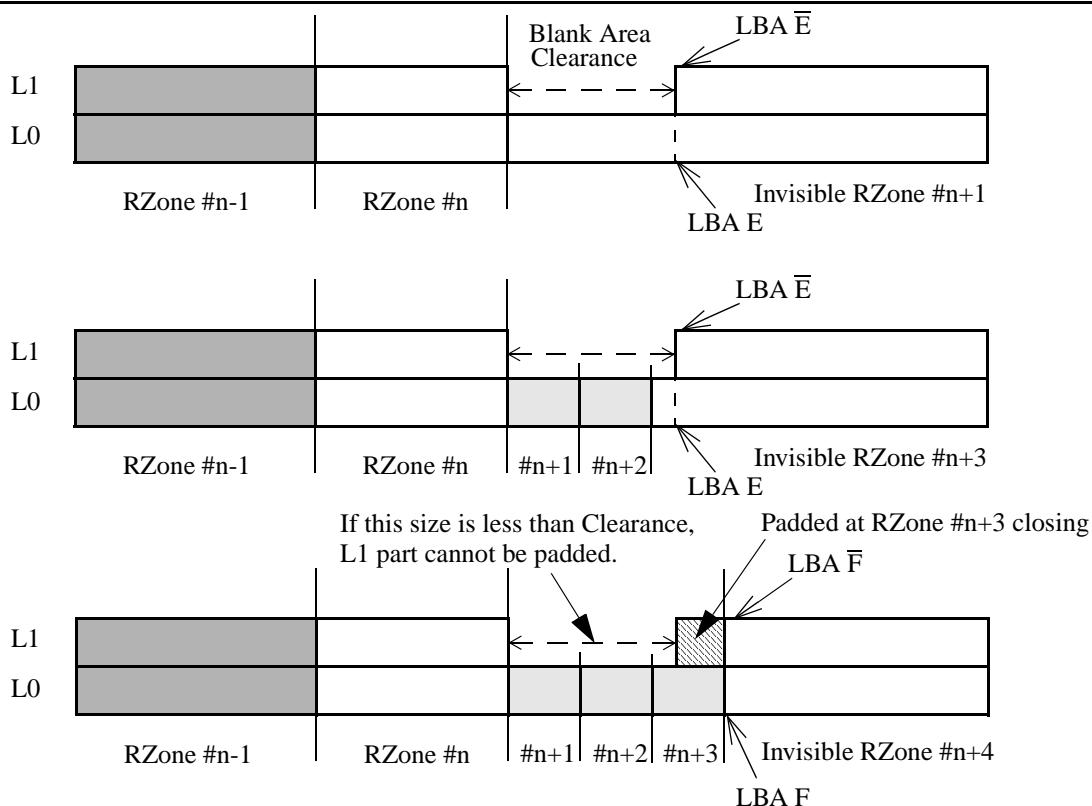
Figure 75 - Invisible RZone shape
