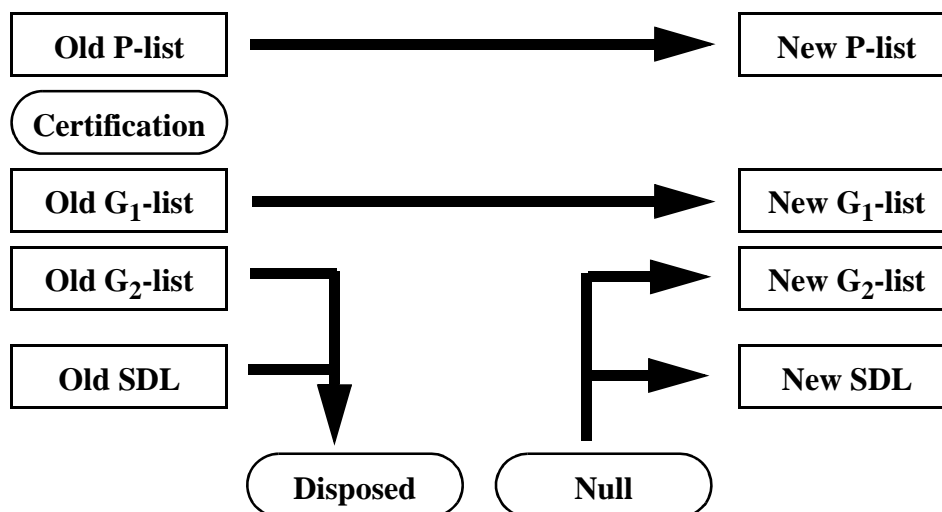
Figure 32 - Formatting Type 4 - Quick Clearing
