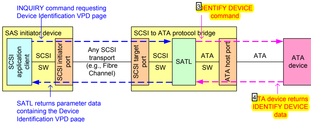
5 Figure 7 — Identification descriptors included by a SATL in a SCSI to ATA protocol bridge
