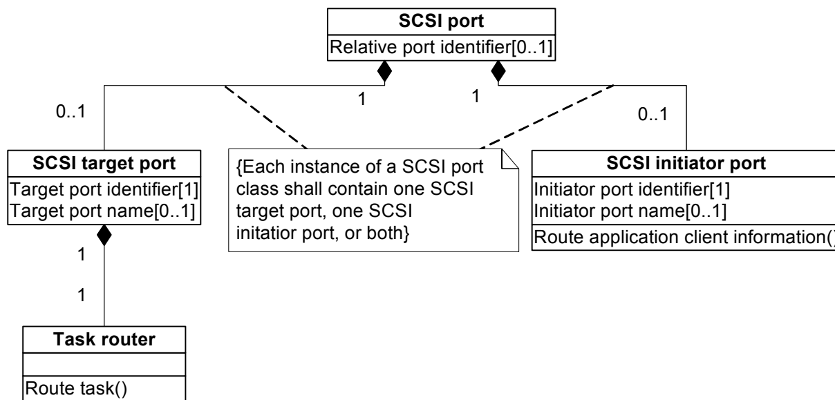
Figure 15 — SCSI port class diagram
