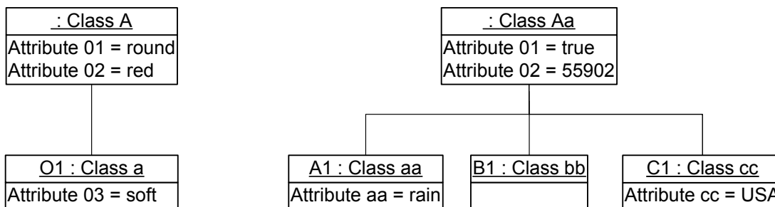
Figure 7 — Notation for link relationships for object diagrams
