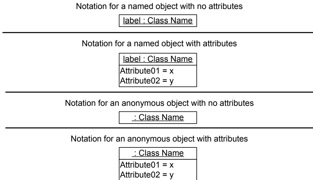
Figure 6 — Object diagram conventions
