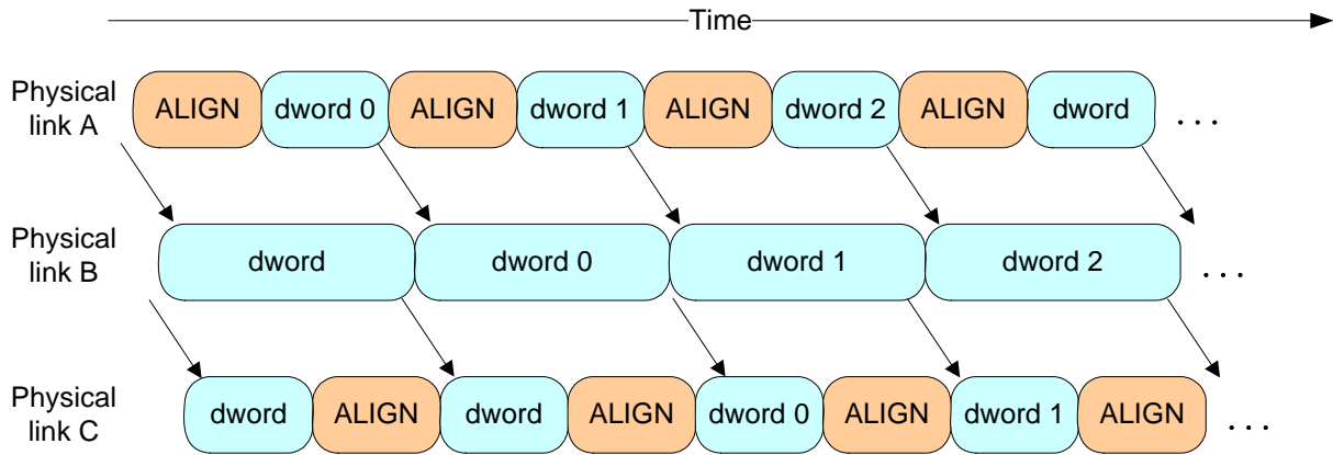
Figure 29 — Rate matching example [changed]
