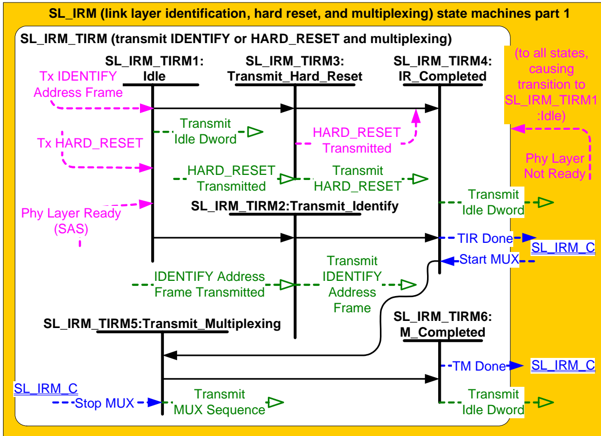
Figure 26 — SL_IRM_TIRM (transmit IDENTIFY or HARD_RESET and multiplexing) state machine
