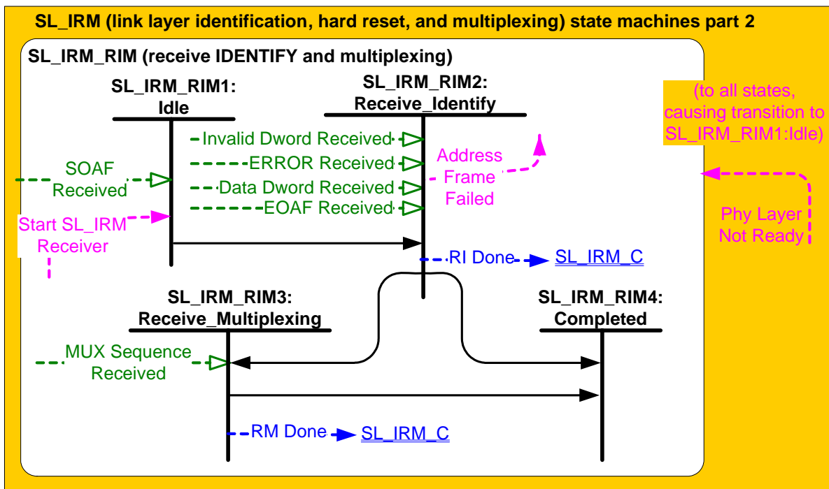
Figure 27 — SL_IRM_RIM (receive IDENTIFY and multiplexing) state machine
