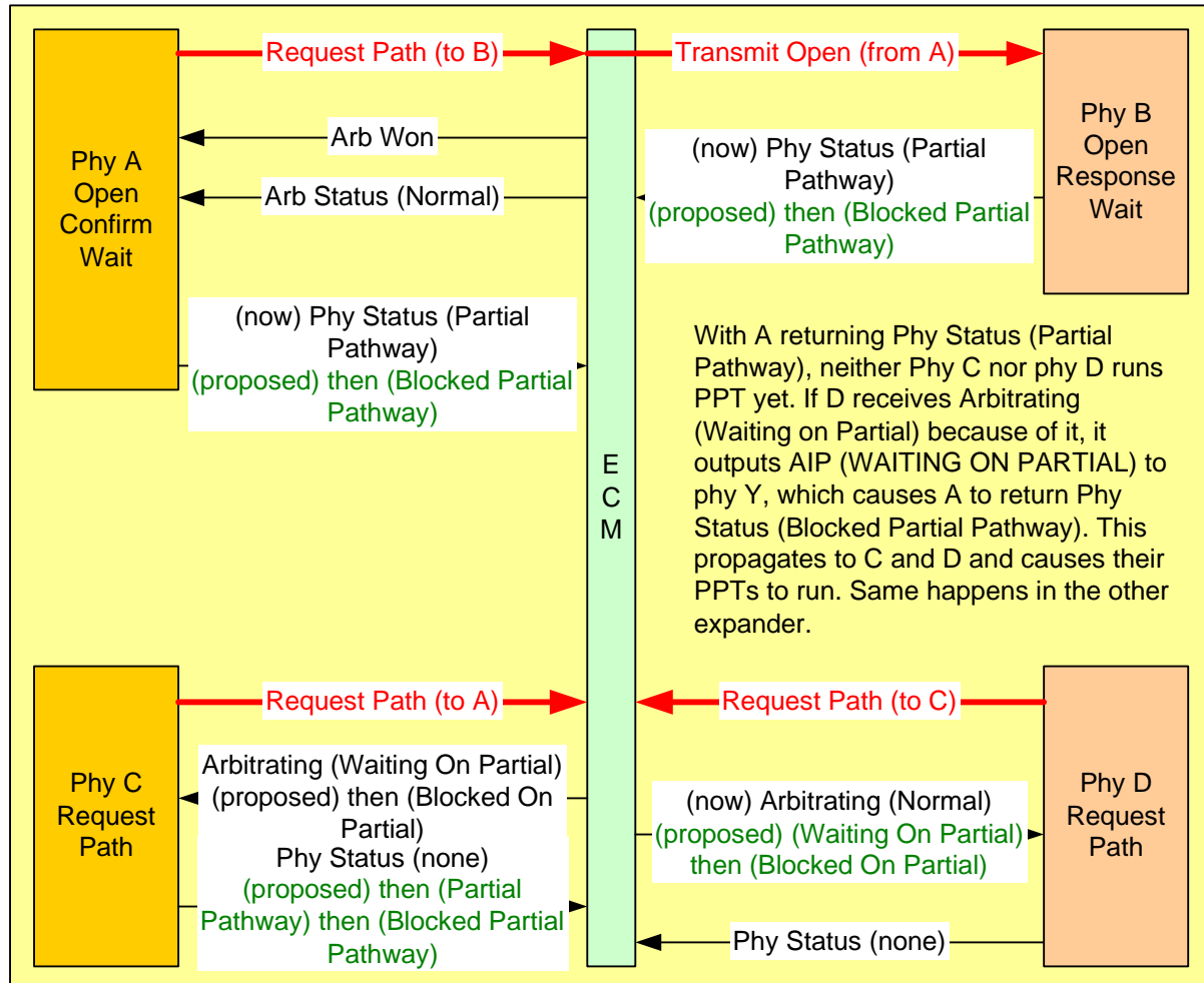
Figure 6 — Forward Phy Status from phy to phy
