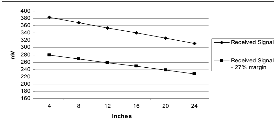
Figure 61: Expected minimum host-side controller receive signal level versus trace length
