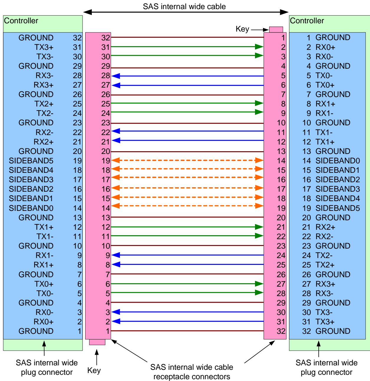
Figure 7 — SAS internal wide cable attaching controller to controller
