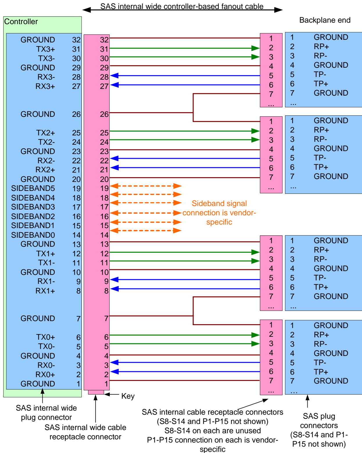
Figure 8 — SAS internal wide controller-based fanout cable
