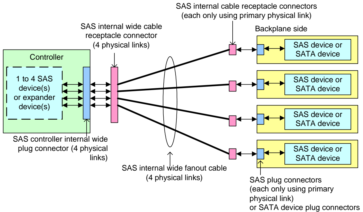
Figure 4 — Internal wide controller-based fanout cable environment
