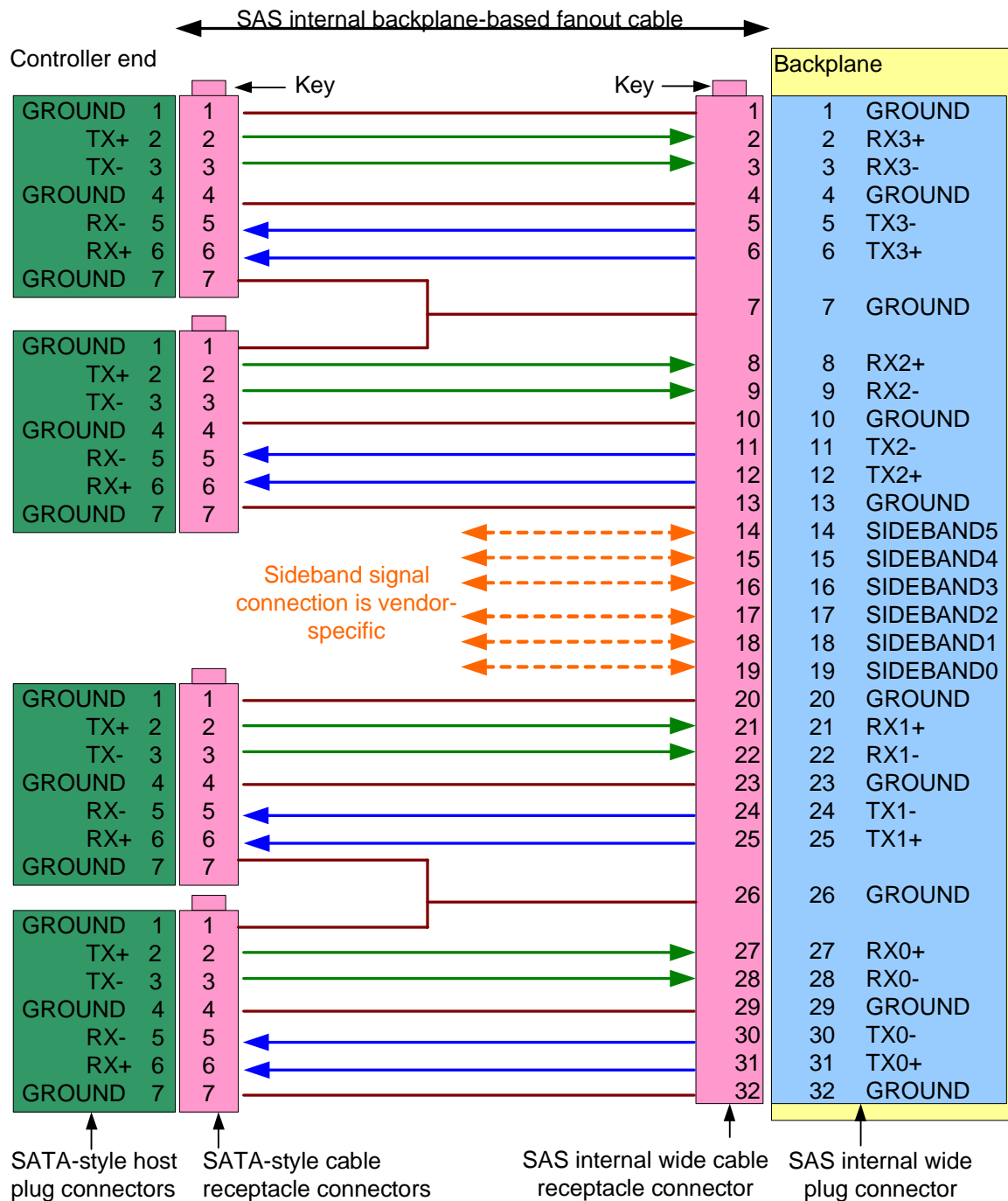
Figure 9 — SAS internal wide backplane-based fanout cable
