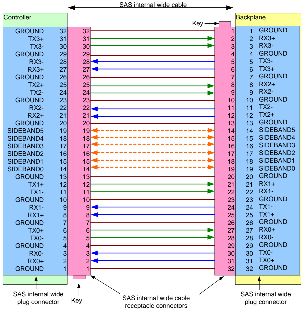
Figure 6 — SAS internal wide cable attaching controller to backplane
