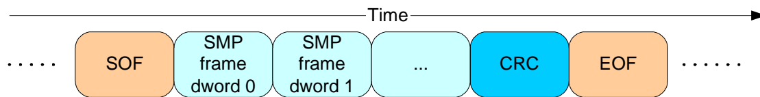
Figure 88 — SMP frame transmission
