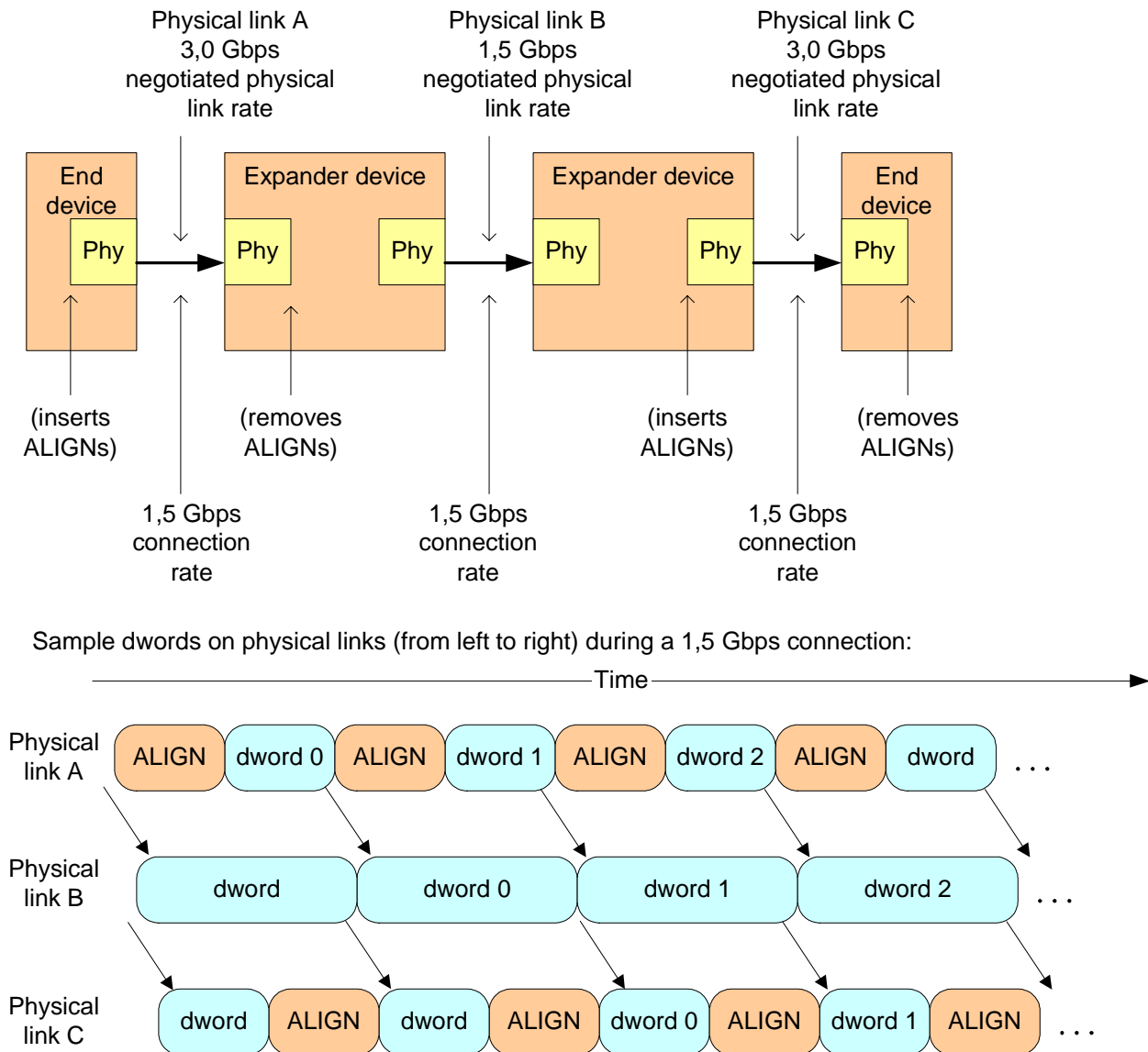
Figure 71 — Rate matching example
