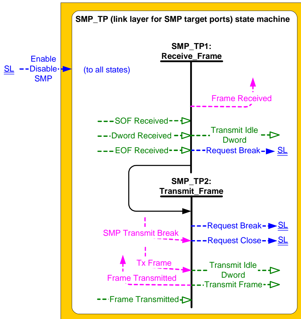
Figure 90 — SMP_TP (link layer for SMP target phys) state machine
