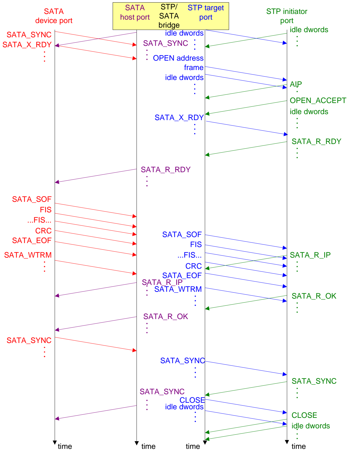
Figure 87 — STP target port opening an STP connection
