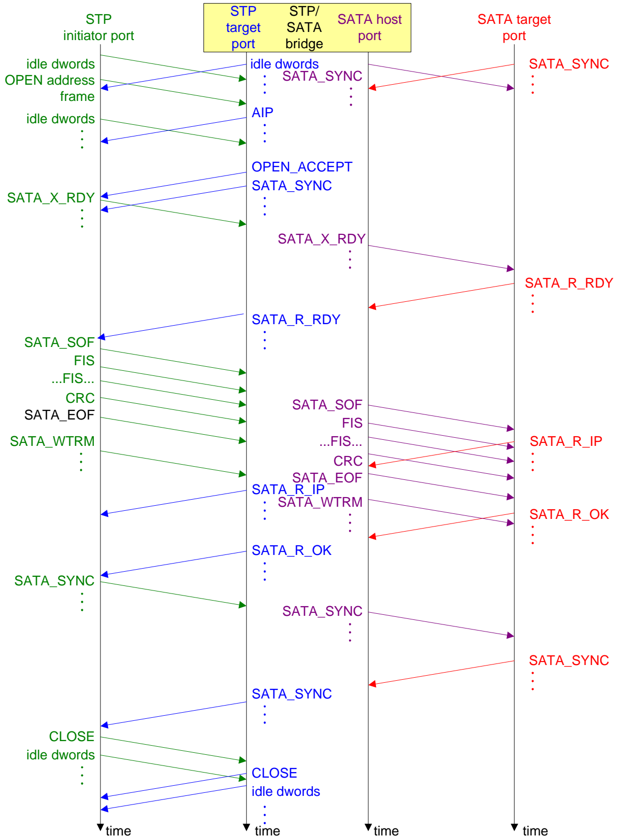
Figure 86 — STP initiator port opening an STP connection
