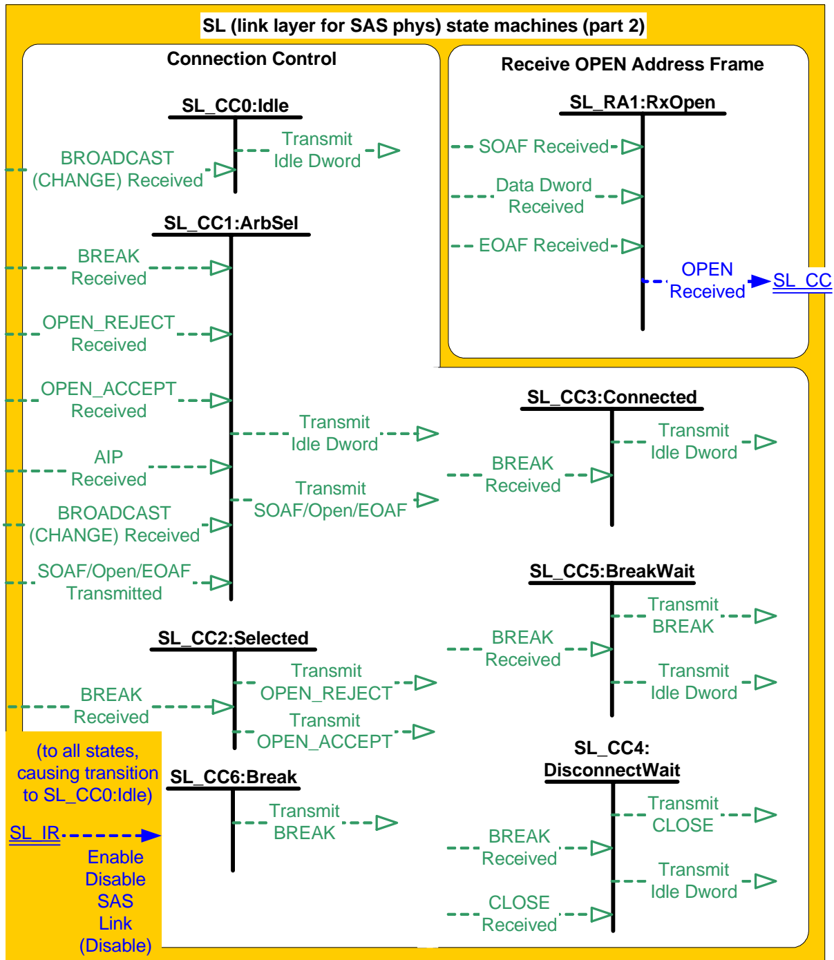
Figure 73 — SL (link layer for SAS phys) state machine (part 2)
