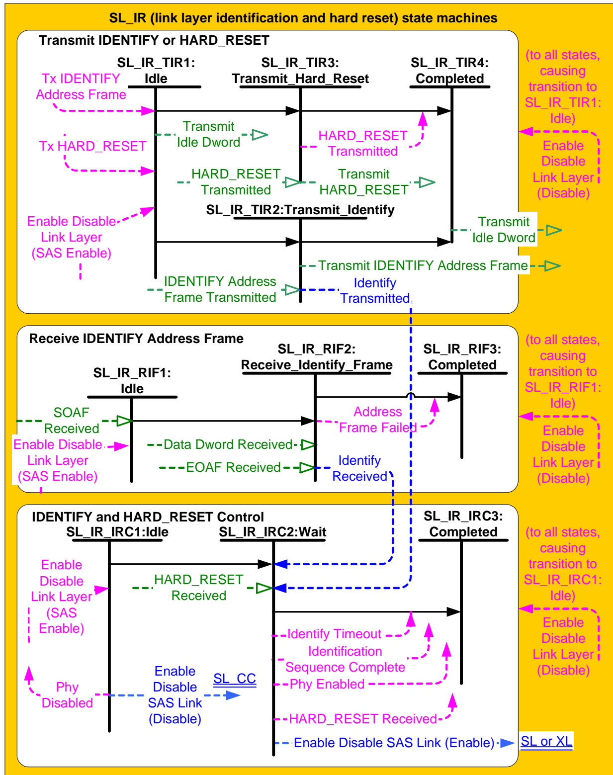
Figure 67 — SL_IR (link layer identification and hard reset) state machines
