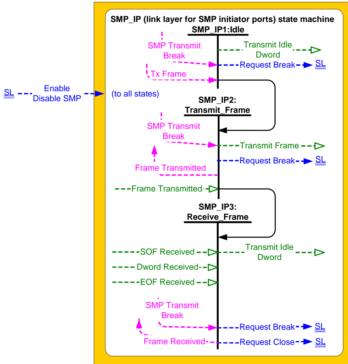
Figure 89 — SMP_IP (link layer for SMP initiator phys) state machine
