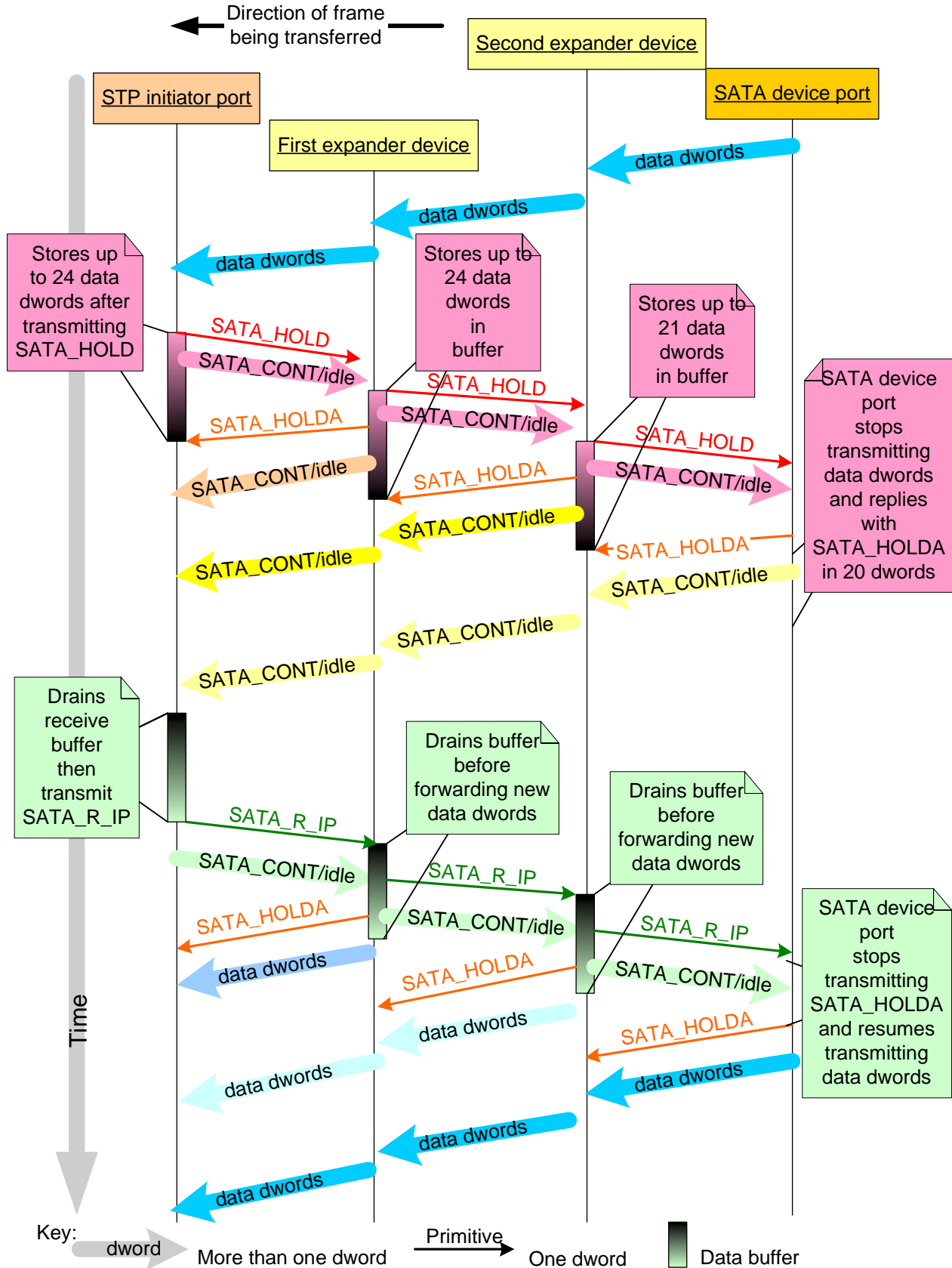
Figure 85 — STP flow control
