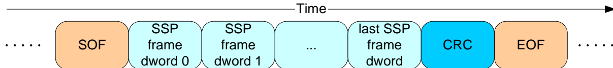
Figure 77 — SSP frame transmission
