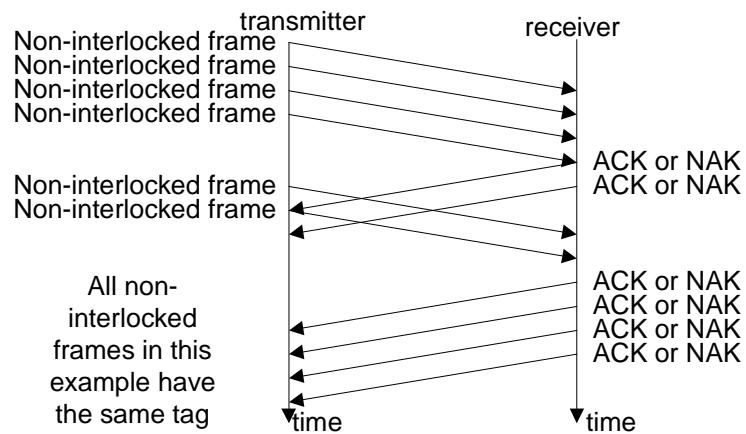
Figure 79 — Non-interlocked frames with the same tag
