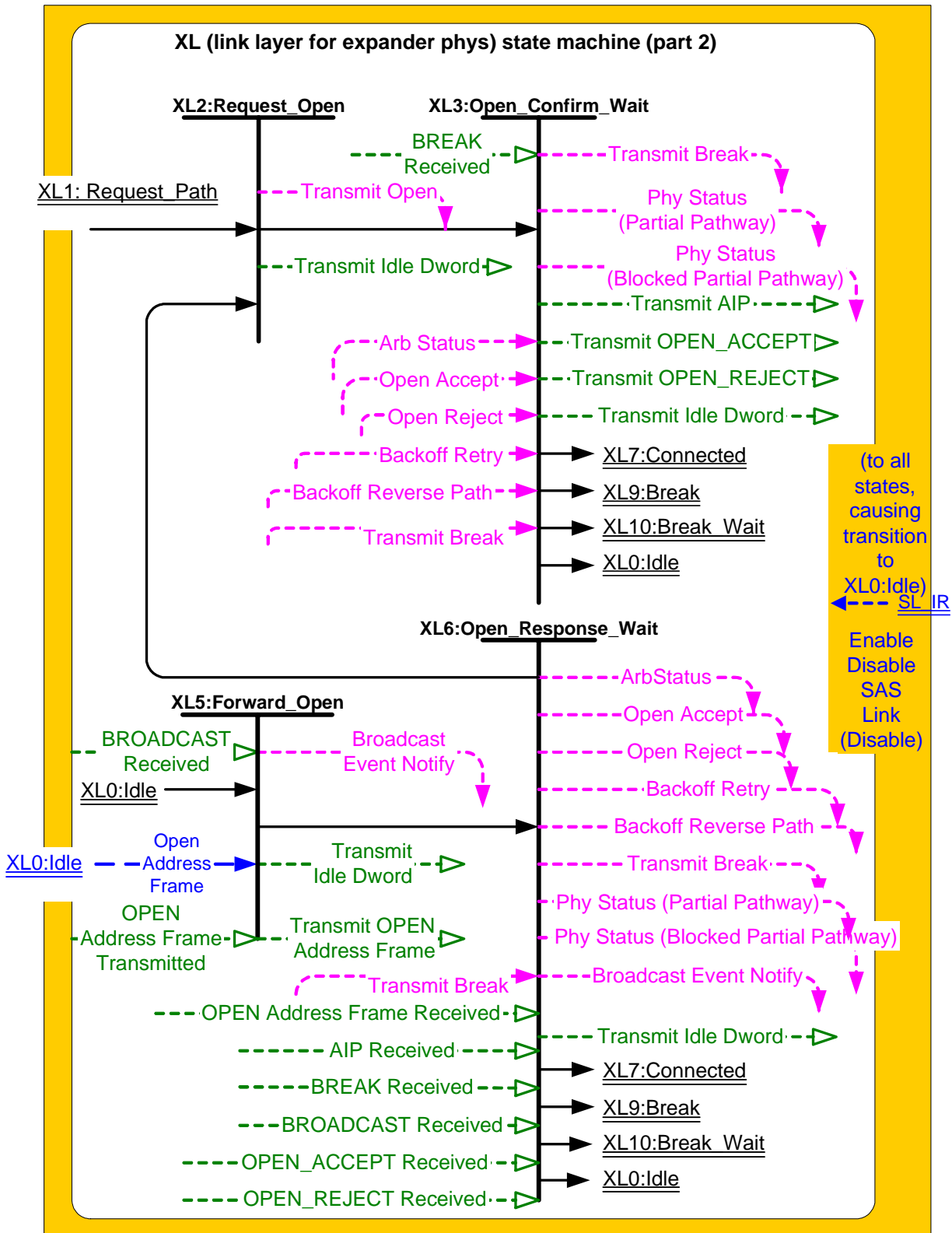
Figure 75 — XL (link layer for expander phys) state machine (part 2)
