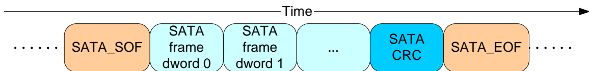
Figure 84 — STP frame transmission
