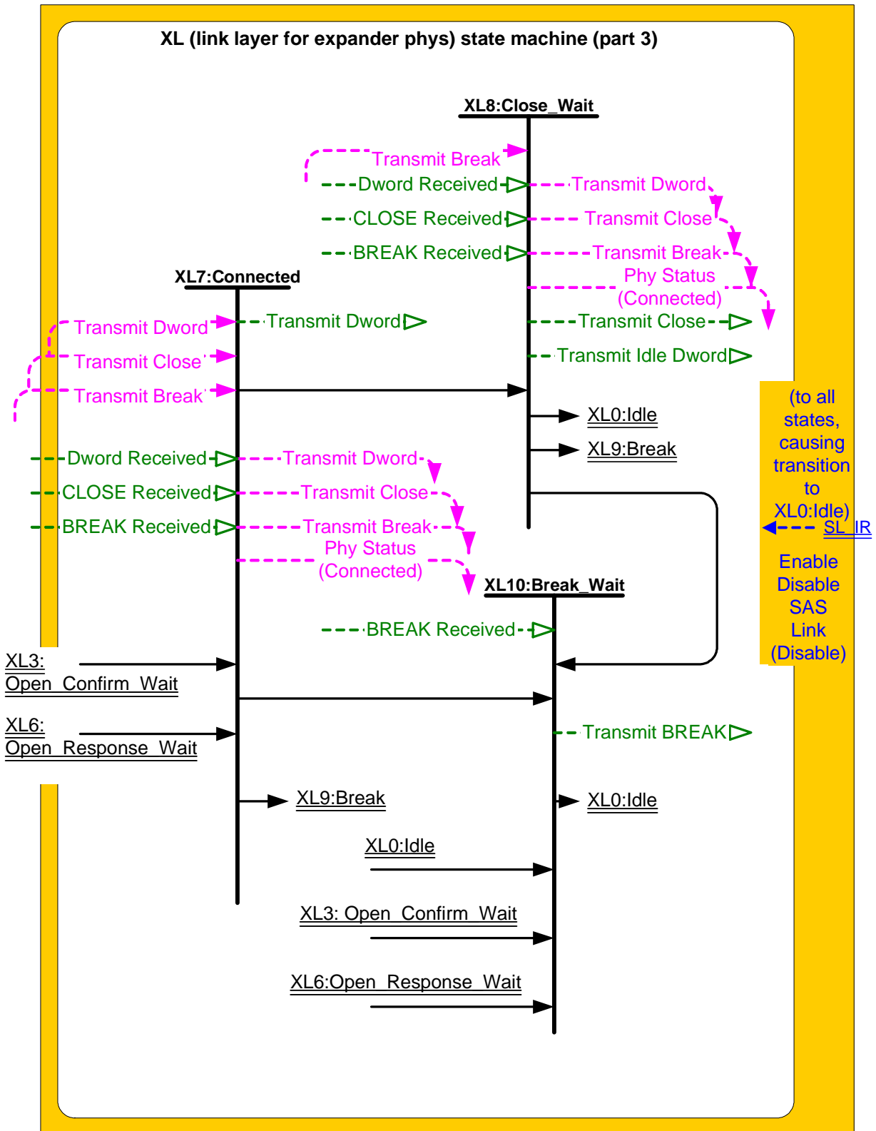
Figure 76 — XL (link layer for expander phys) state machine (part 3)
