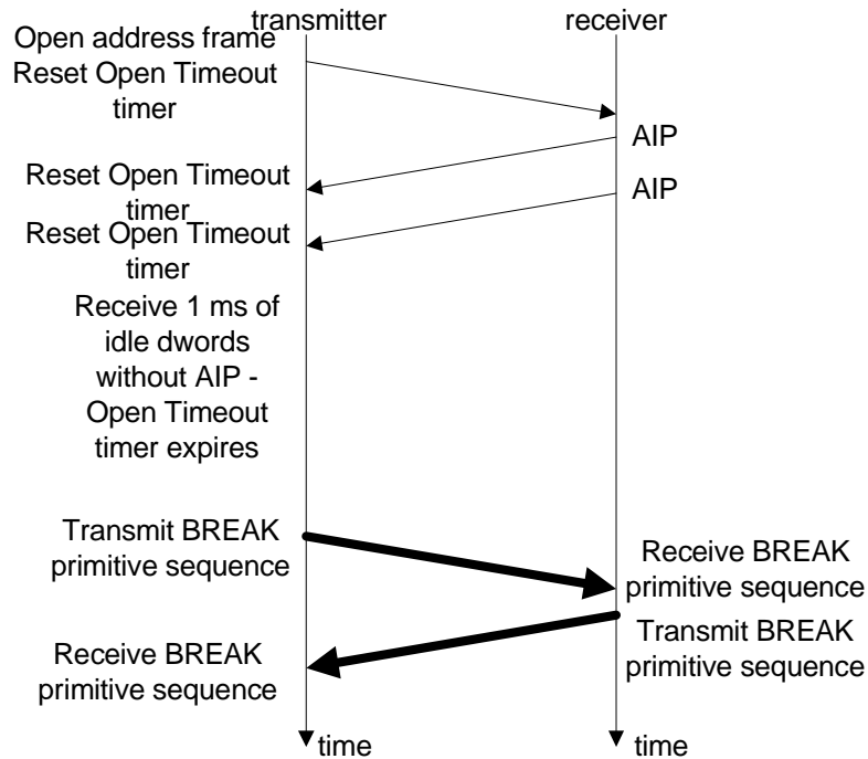
Figure 69 — Connection request timeout example
