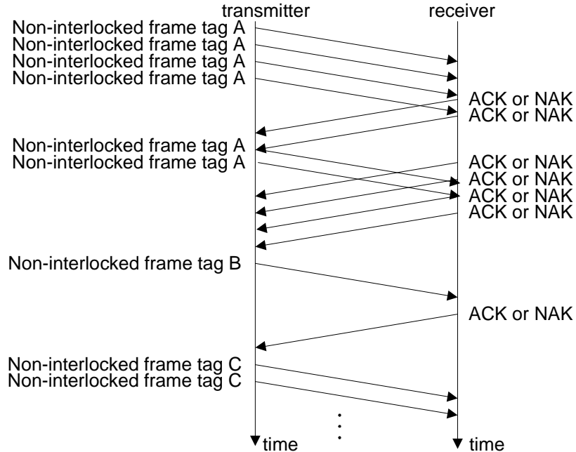
Figure 80 — Non-interlocked frames with different tags
