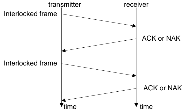
Figure 78 — Interlocked frames
