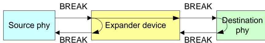
Figure 68 — BREAK usage
