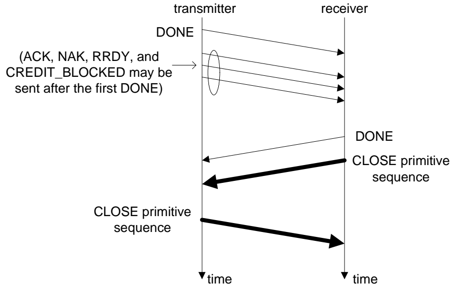
Figure 81 — Closing an SSP connection example
