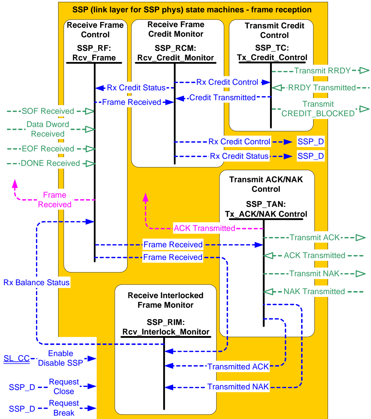
Figure 83 — SSP (link layer for SSP phys) state machines (part 2 - frame reception)
