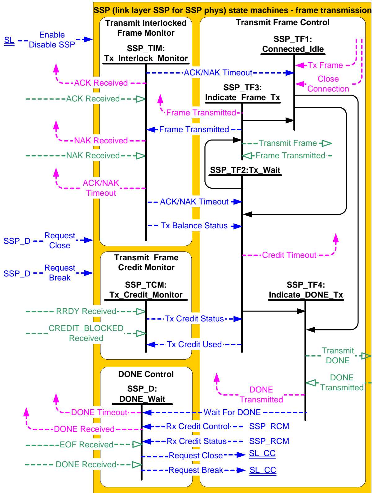
Figure 82 — SSP (link layer for SSP phys) state machines (part 1 - frame transmission)
