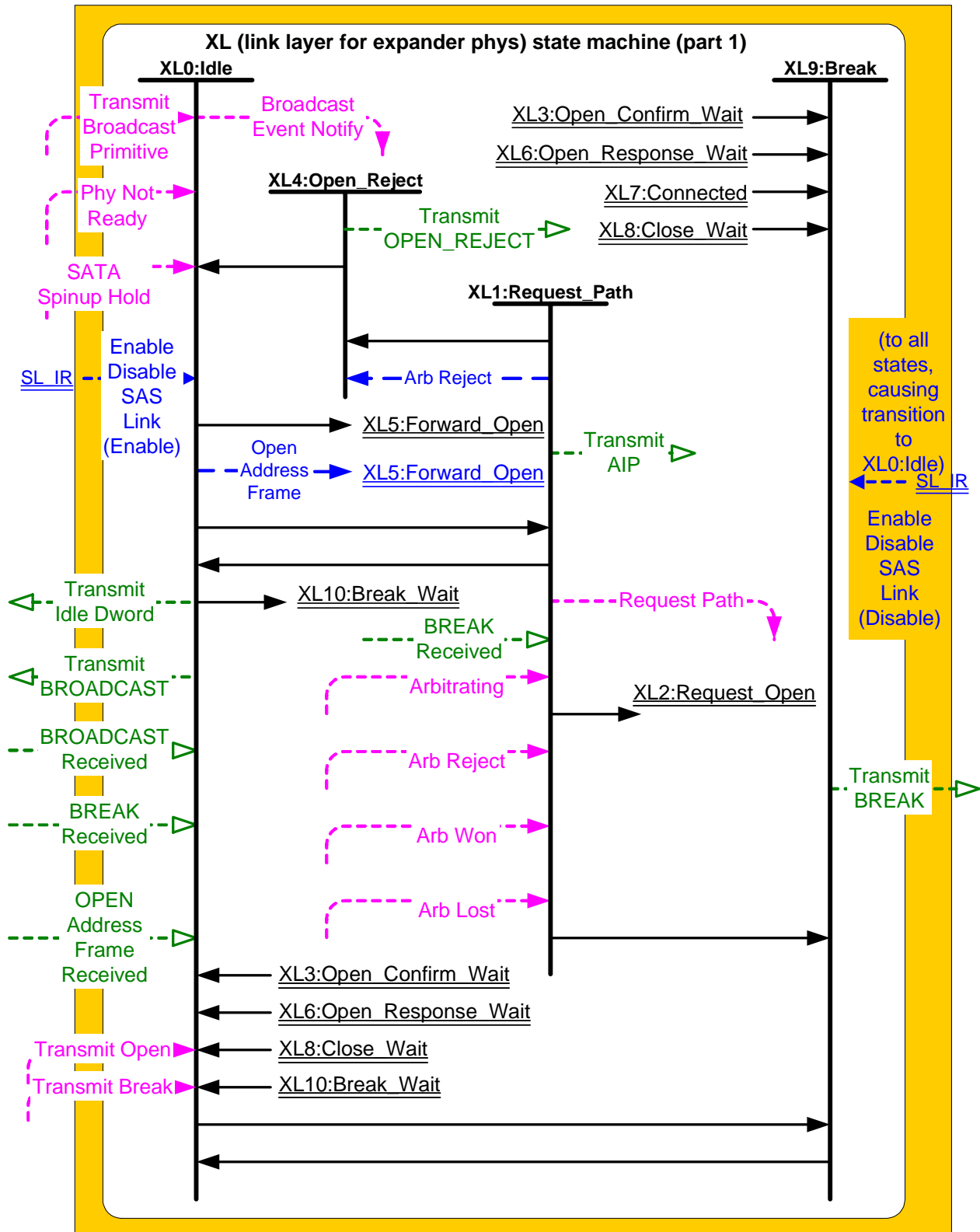
Figure 74 — XL (link layer for expander phys) state machine (part 1)
