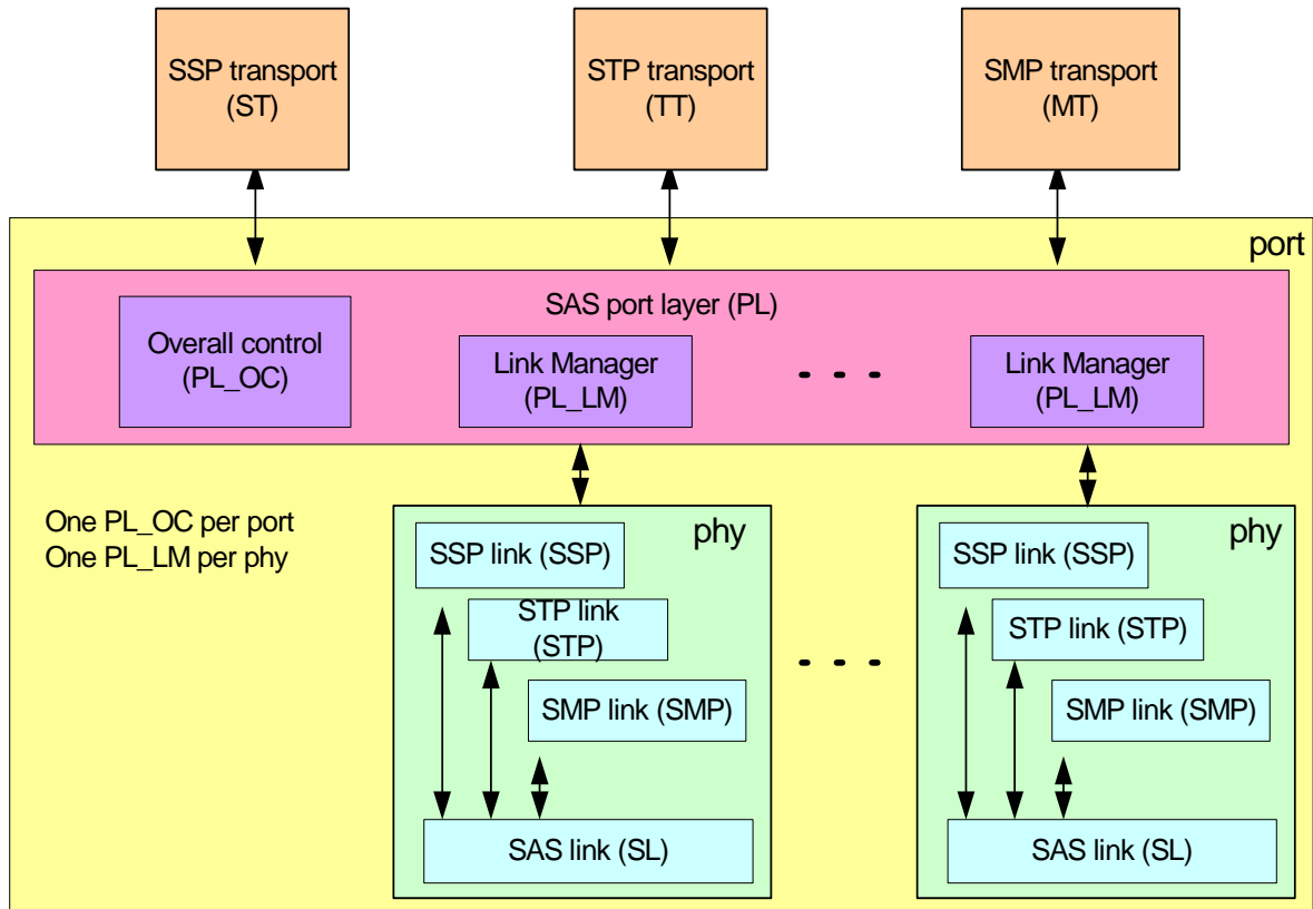
Figure 1. SAS port layer position
