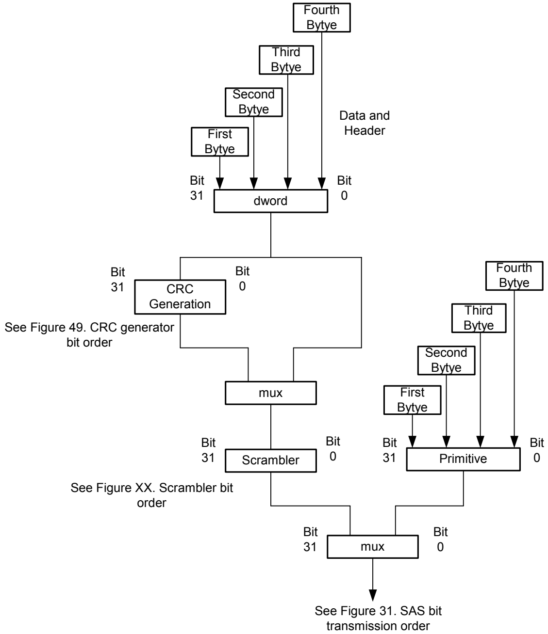
Figure 2 – Port transmit path
