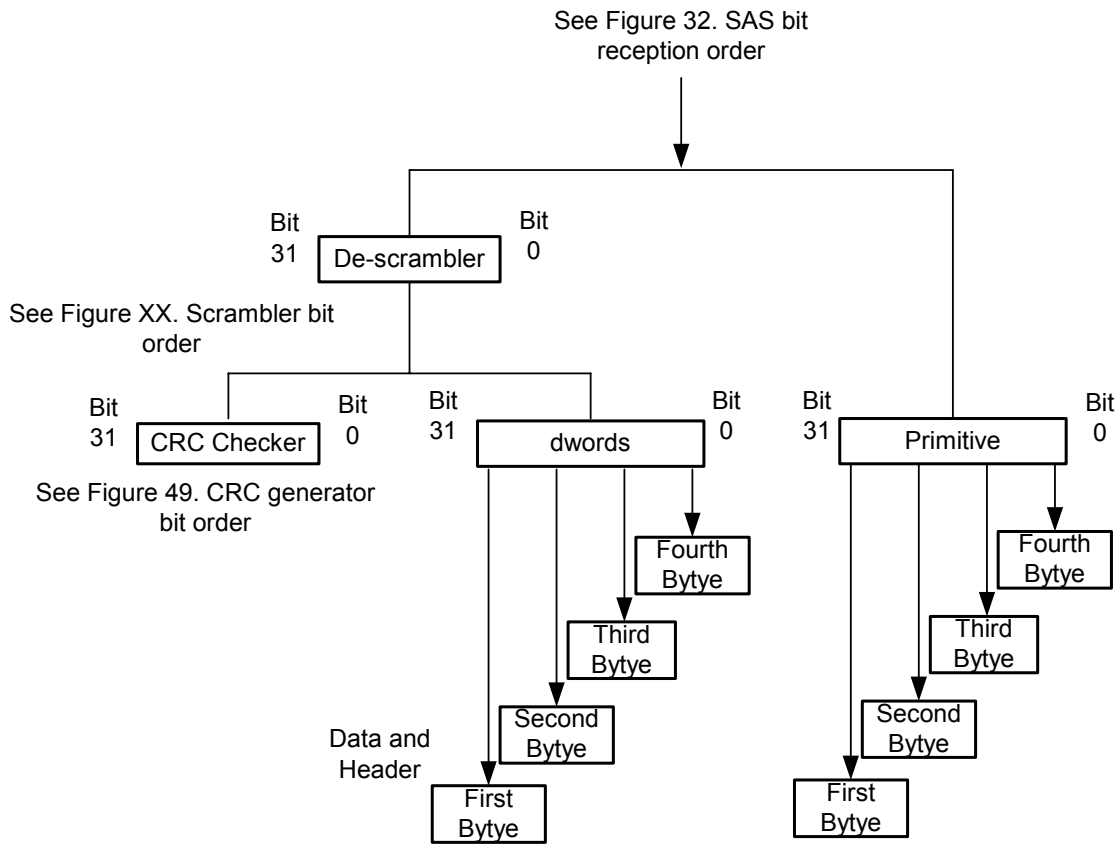
Figure 1 – Port receive path
