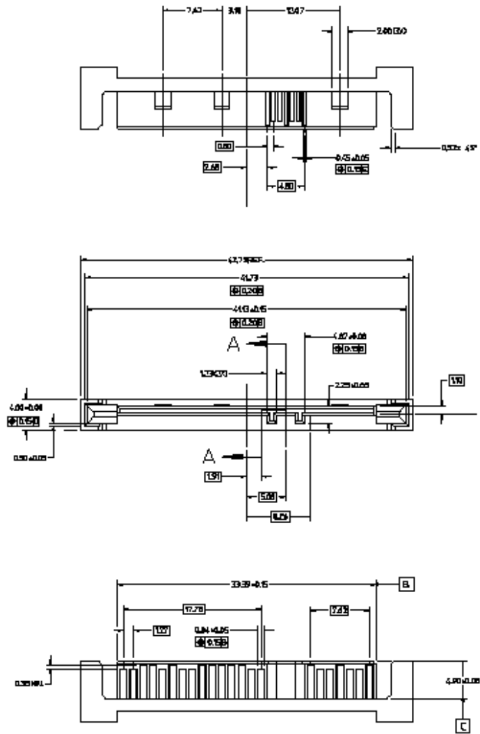
Plug connector.
