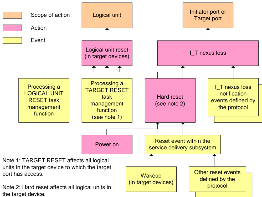
Figure 1. Power on, hard reset, logical unit, and I_T nexus loss relationships
