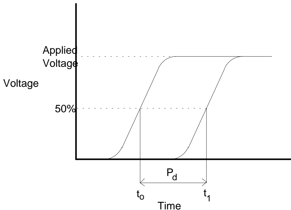
Figure 3 - Propagation time measurements
