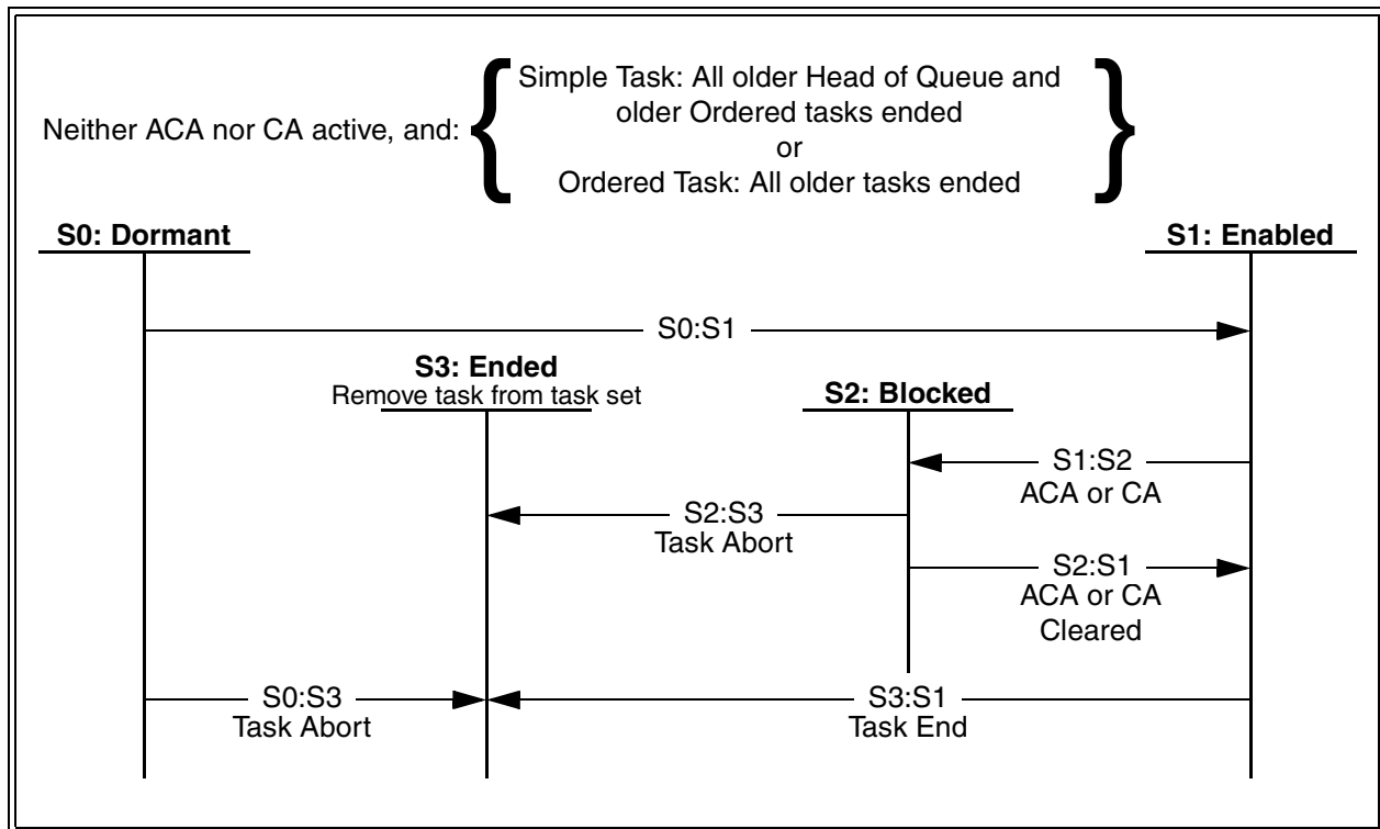
Figure 33 — Task states
