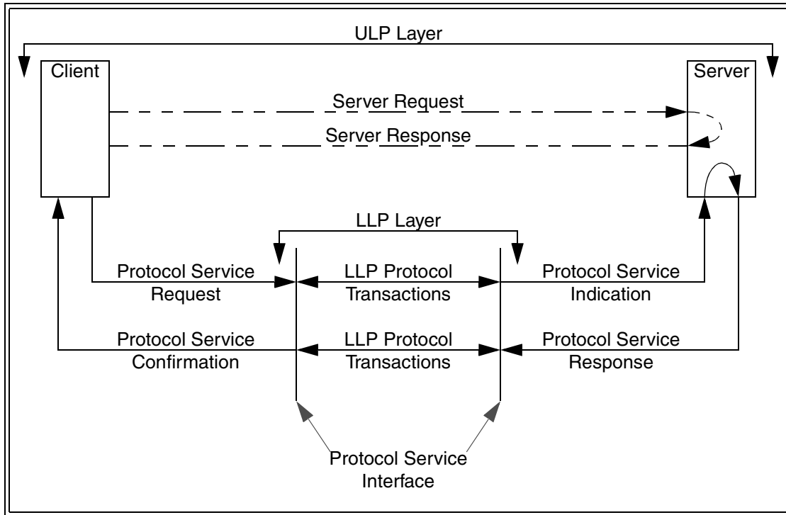
Figure 27 — Request-Response ULP transaction and related LLP services
