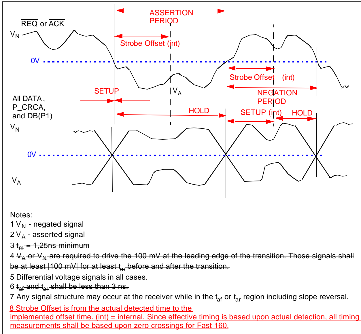
Figure 42 - LVD timing measurement points for DT = Fast - 160 data transfers
