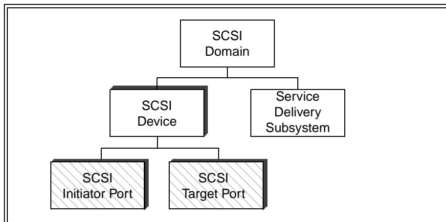
Figure 4 — Domain hierarchy
